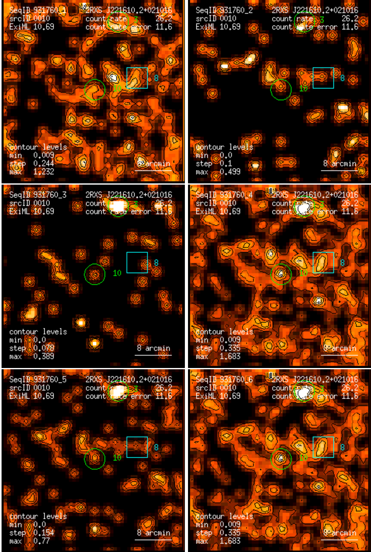
Figure 10: RASS 931760: detection 0010: band rate images, Gaussian filter: (1) PSPC channels 11 – 41, (2) 52 – 90, (3) 91 – 201, (4) 11 – 235, (5) 52 – 201, (6) 11 – 201. Broad band rates in counts/ks. Band rate contour levels in counts/ks/arcmin 2 .
