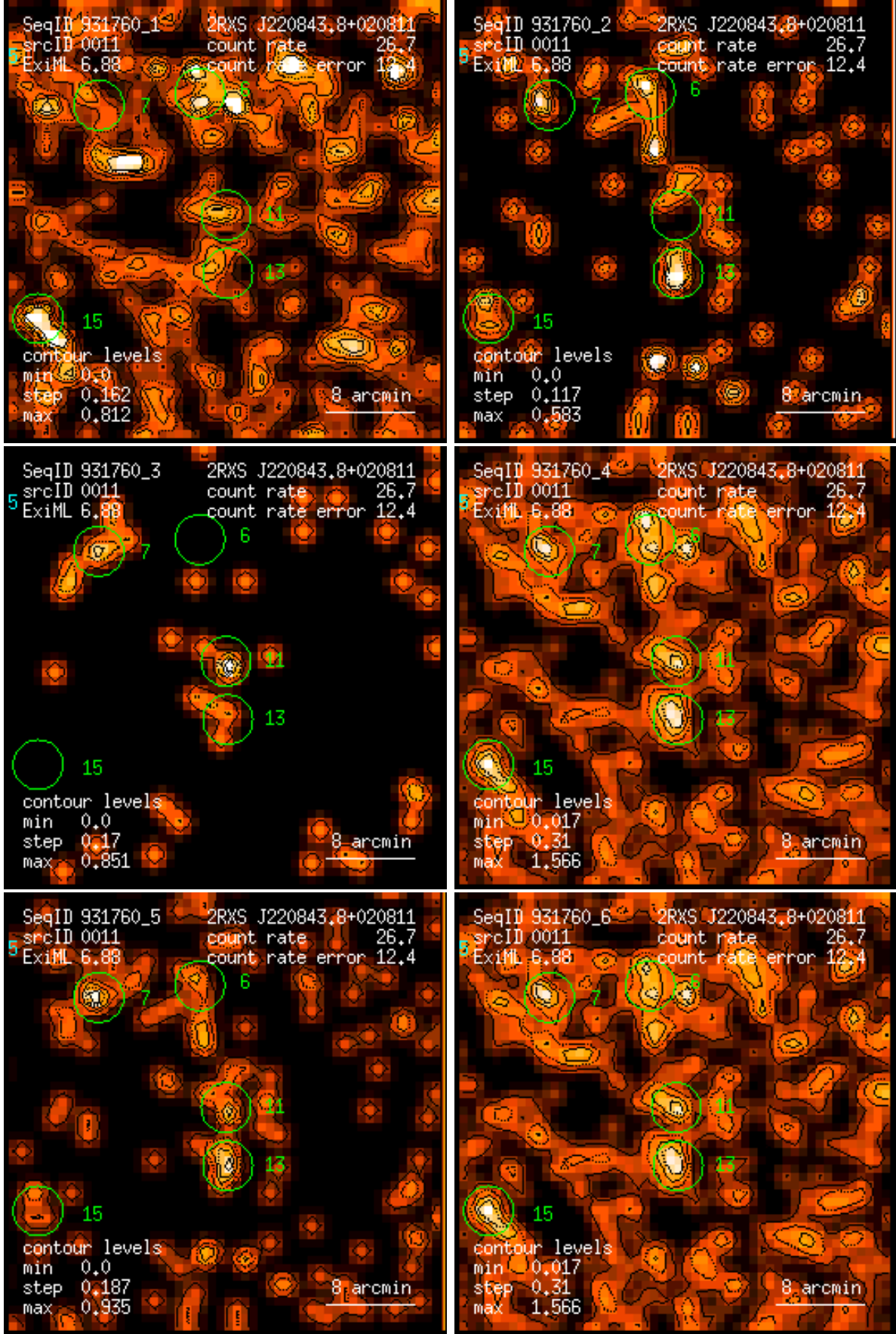
Figure 11: RASS 931760: detection 0011: band rate images, Gaussian filter: (1) PSPC channels 11 – 41, (2) 52 – 90, (3) 91 – 201, (4) 11 – 235, (5) 52 – 201, (6) 11 – 201. Broad band rates in counts/ks. Band rate contour levels in counts/ks/arcmin 2 .
