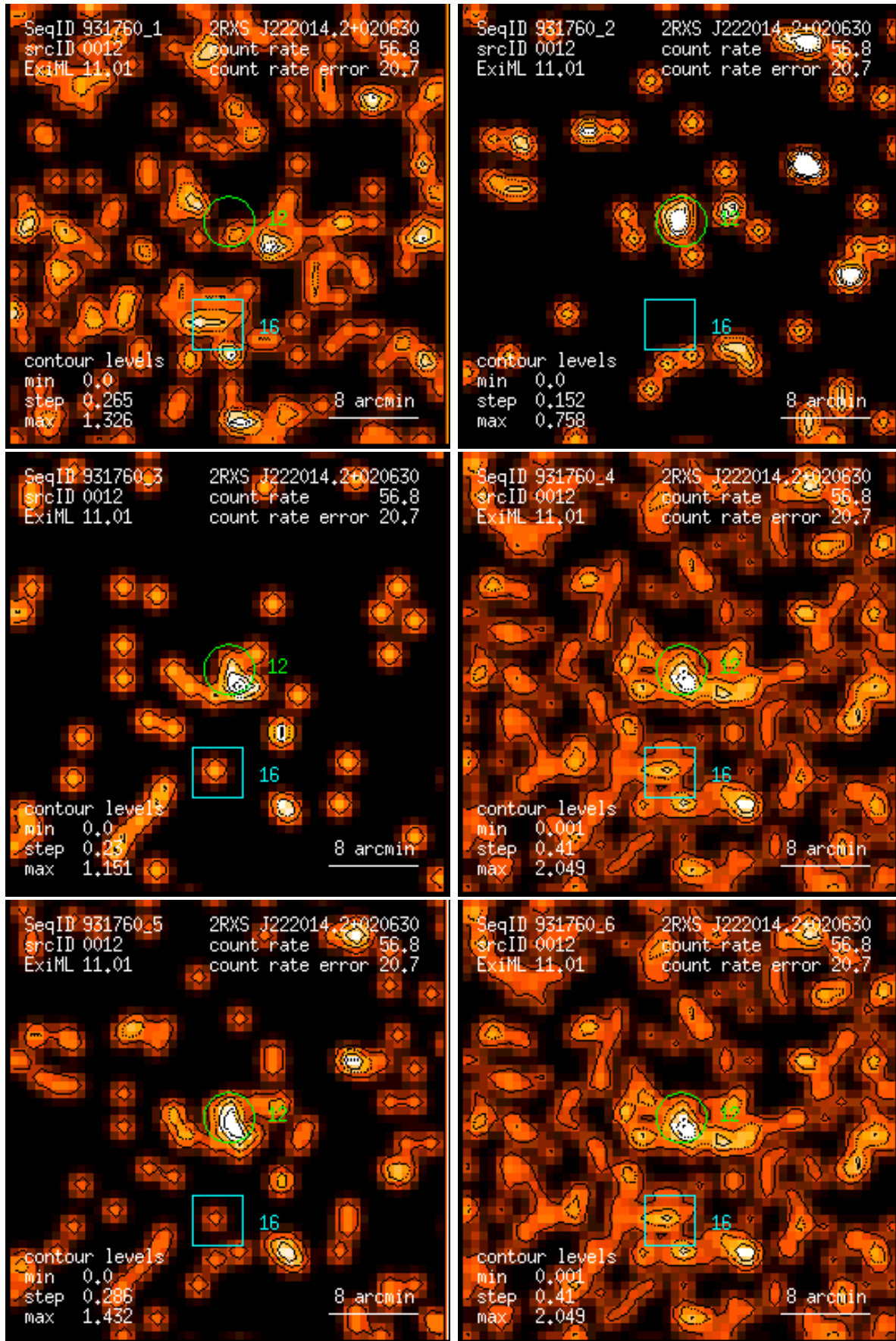
Figure 12: RASS 931760: detection 0012: band rate images, Gaussian filter: (1) PSPC channels 11 – 41, (2) 52 – 90, (3) 91 – 201, (4) 11 – 235, (5) 52 – 201, (6) 11 – 201. Broad band rates in counts/ks. Band rate contour levels in counts/ks/arcmin 2 .
