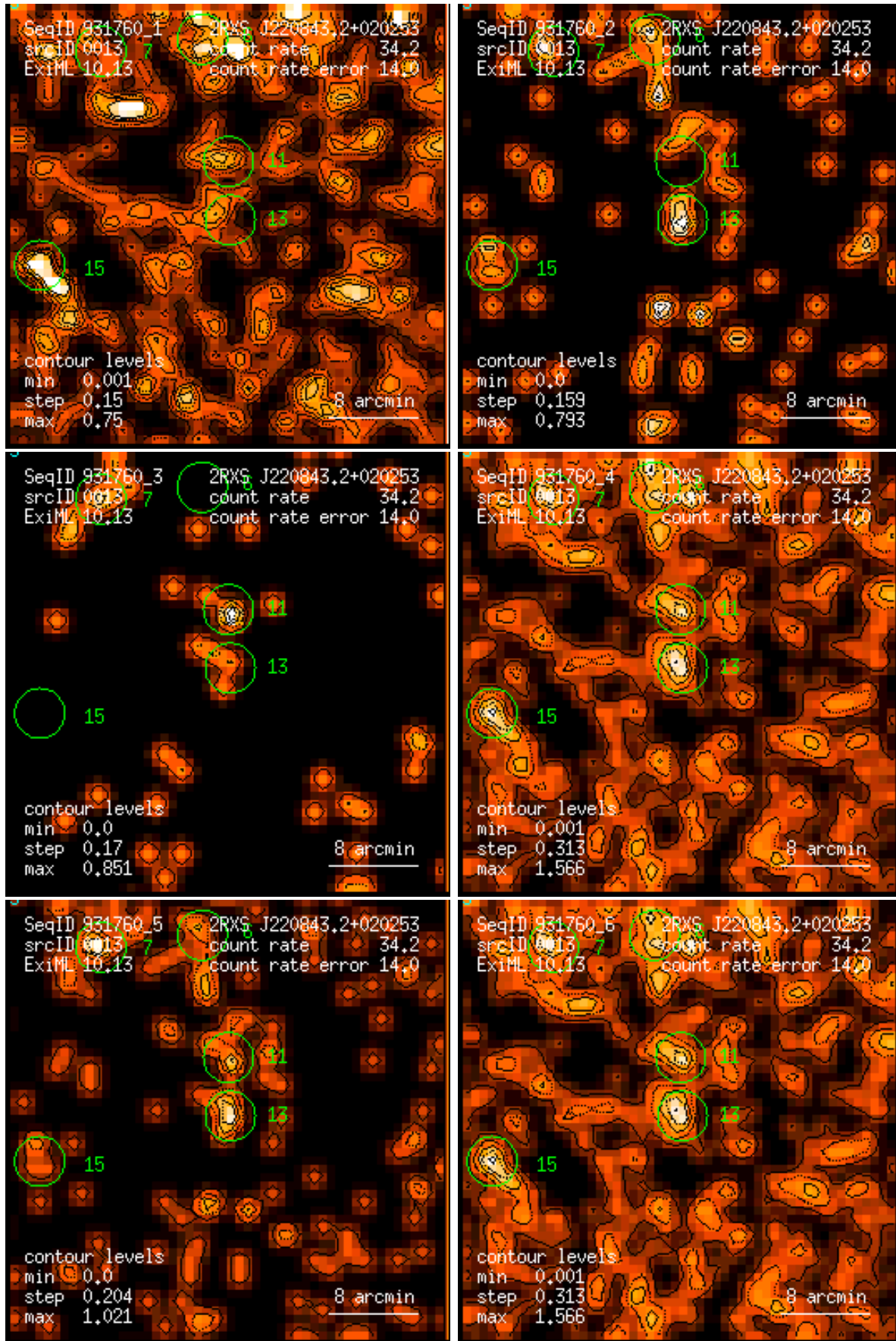
Figure 13: RASS 931760: detection 0013: band rate images, Gaussian filter: (1) PSPC channels 11 – 41, (2) 52 – 90, (3) 91 – 201, (4) 11 – 235, (5) 52 – 201, (6) 11 – 201. Broad band rates in counts/ks. Band rate contour levels in counts/ks/arcmin 2 .
