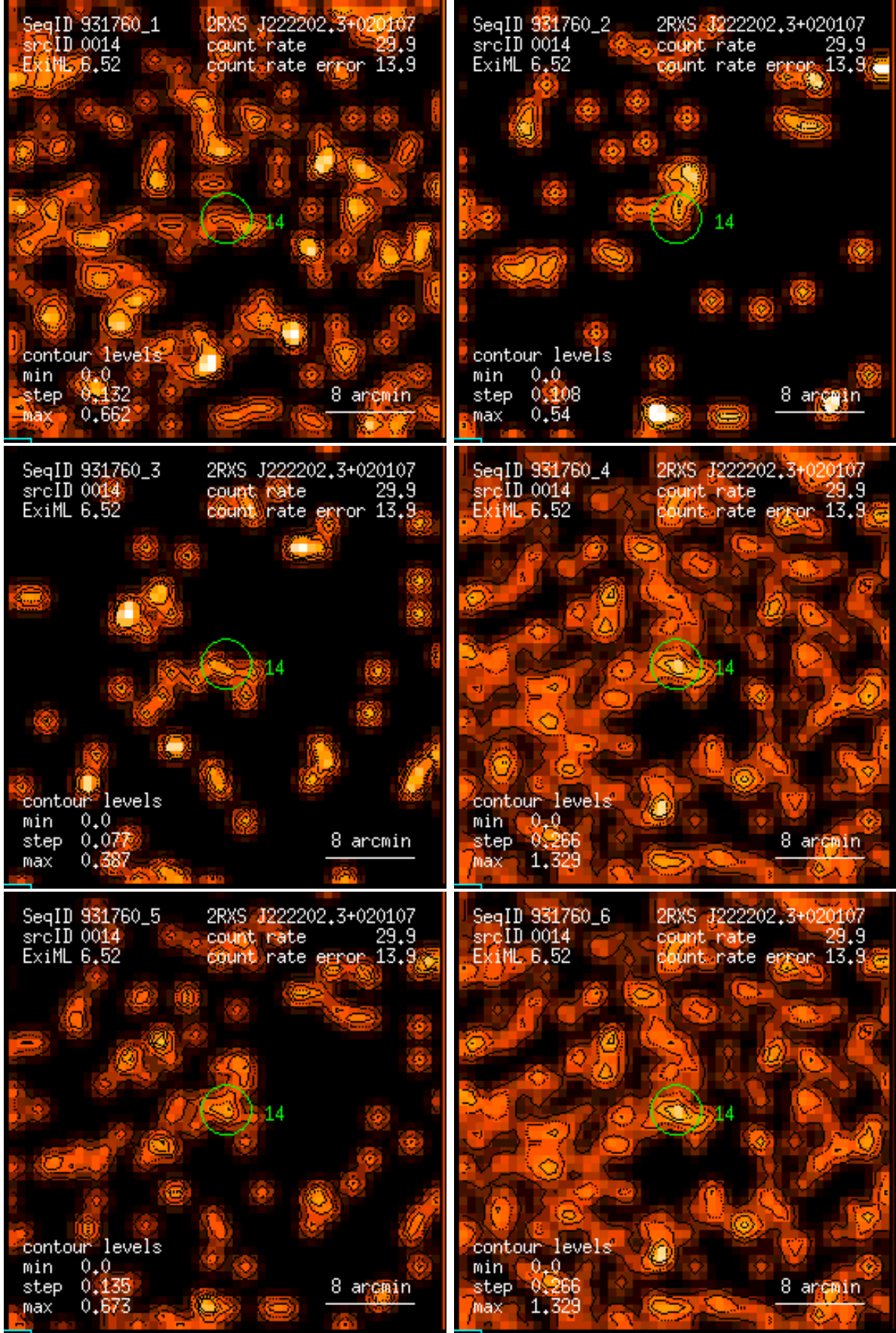
Figure 14: RASS 931760: detection 0014: band rate images, Gaussian filter: (1) PSPC channels 11 – 41, (2) 52 – 90, (3) 91 – 201, (4) 11 – 235, (5) 52 – 201, (6) 11 – 201. Broad band rates in counts/ks. Band rate contour levels in counts/ks/arcmin 2 .
