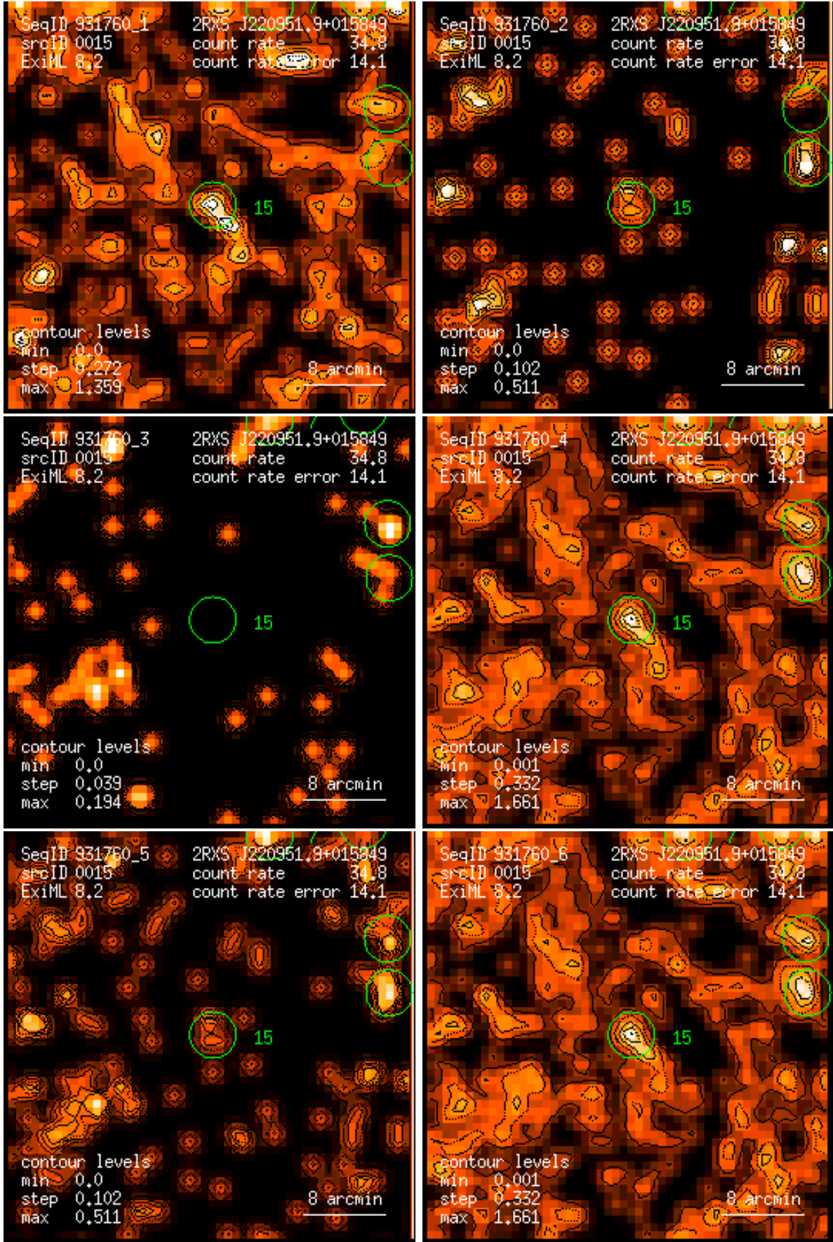
Figure 15: RASS 931760: detection 0015: band rate images, Gaussian filter: (1) PSPC channels 11 – 41, (2) 52 – 90, (3) 91 – 201, (4) 11 – 235, (5) 52 – 201, (6) 11 – 201. Broad band rates in counts/ks. Band rate contour levels in counts/ks/arcmin 2 .
