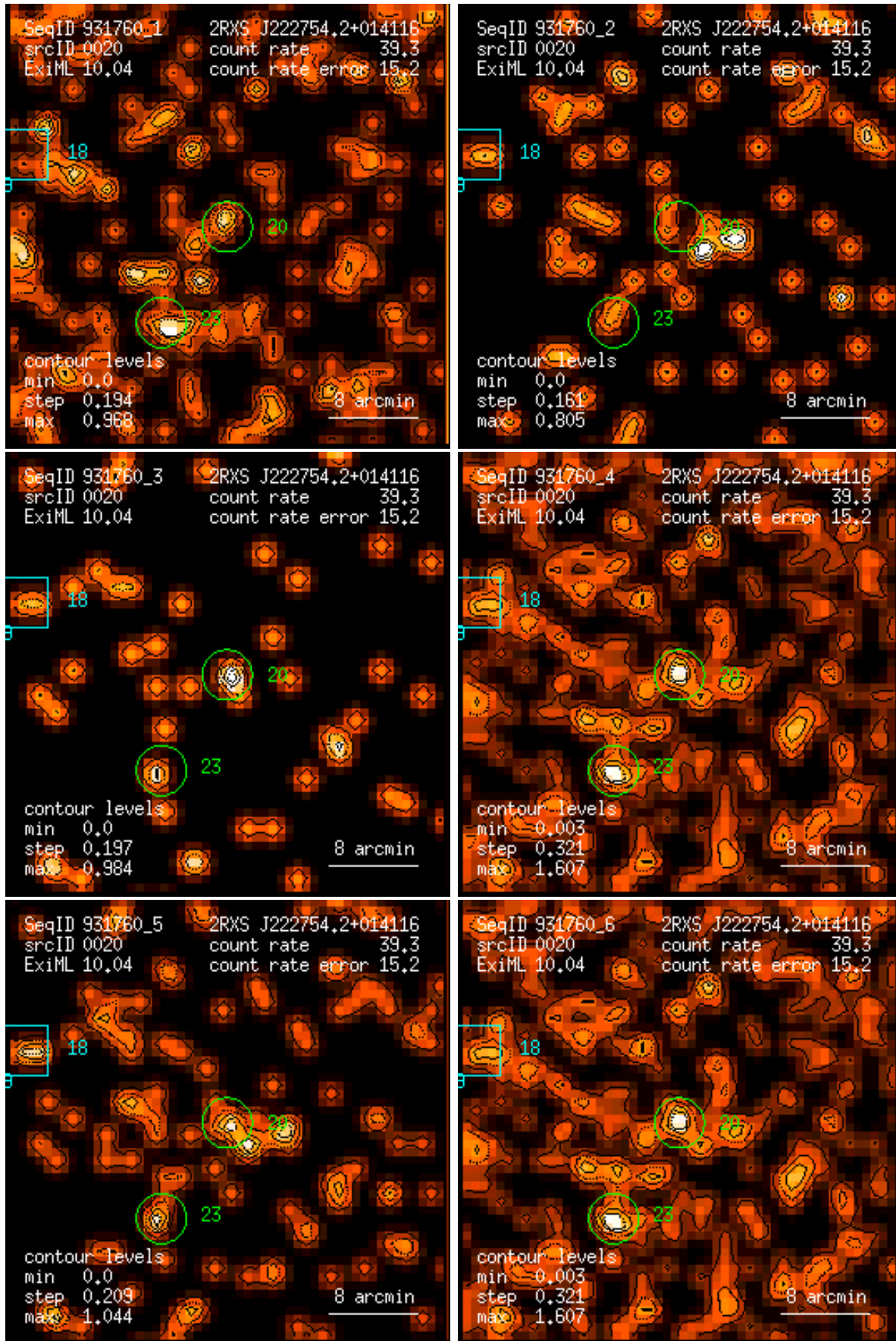
Figure 20: RASS 931760: detection 0020: band rate images, Gaussian filter: (1) PSPC channels 11 – 41, (2) 52 – 90, (3) 91 – 201, (4) 11 – 235, (5) 52 – 201, (6) 11 – 201. Broad band rates in counts/ks. Band rate contour levels in counts/ks/arcmin 2 .
