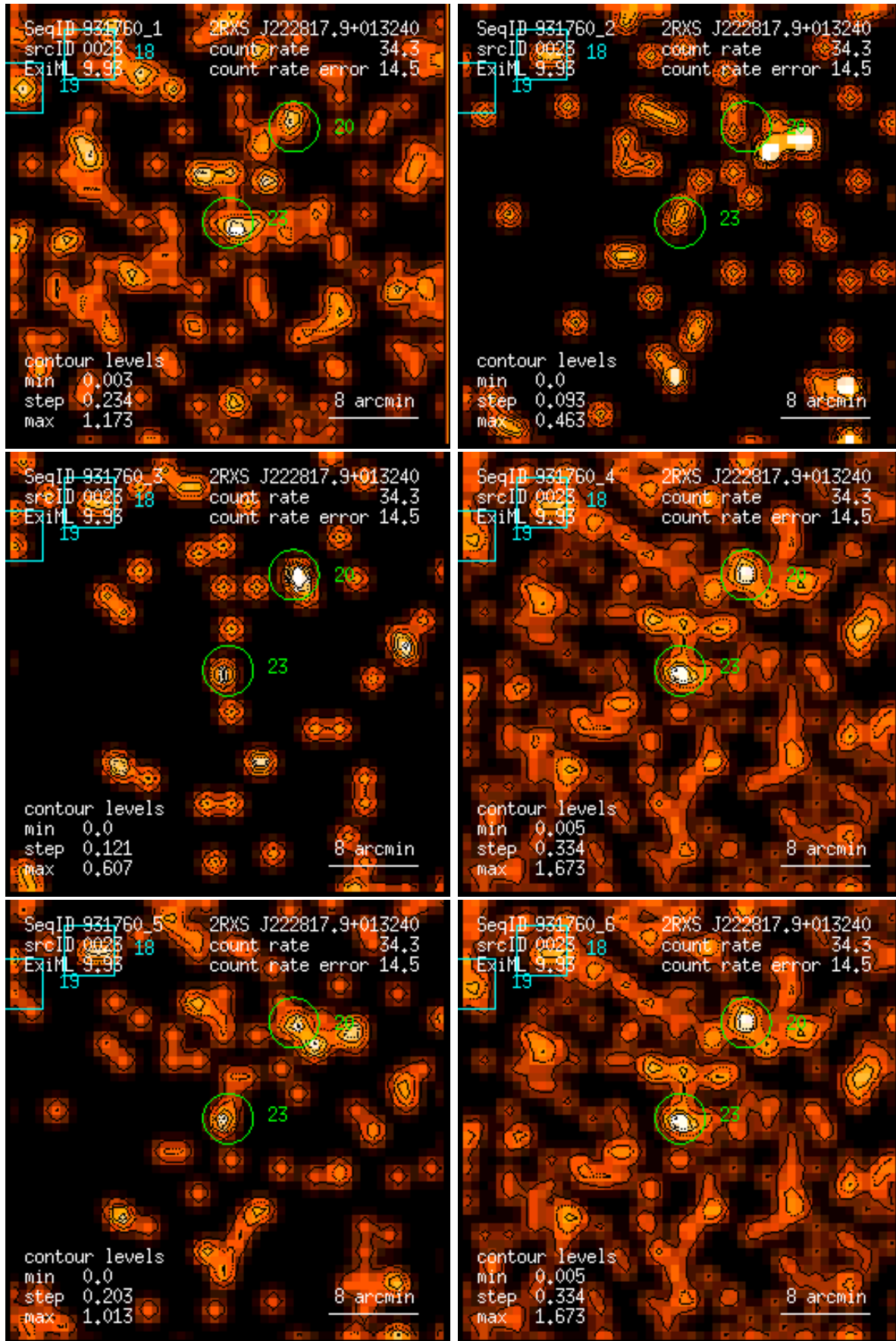
Figure 23: RASS 931760: detection 0023: band rate images, Gaussian filter: (1) PSPC channels 11 – 41, (2) 52 – 90, (3) 91 – 201, (4) 11 – 235, (5) 52 – 201, (6) 11 – 201. Broad band rates in counts/ks. Band rate contour levels in counts/ks/arcmin 2 .
