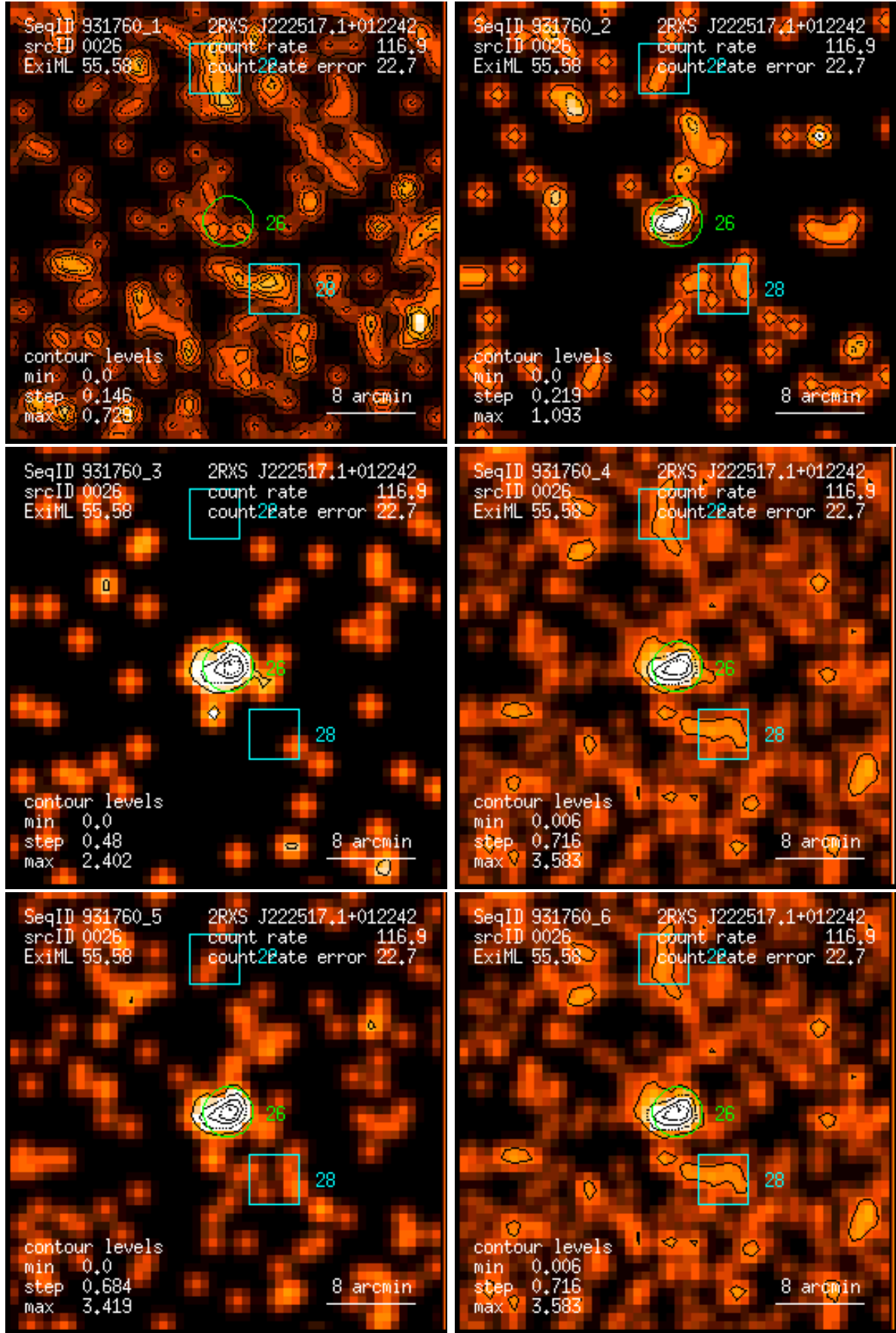
Figure 26: RASS 931760: detection 0026: band rate images, Gaussian filter: (1) PSPC channels 11 – 41, (2) 52 – 90, (3) 91 – 201, (4) 11 – 235, (5) 52 – 201, (6) 11 – 201. Broad band rates in counts/ks. Band rate contour levels in counts/ks/arcmin 2 .
