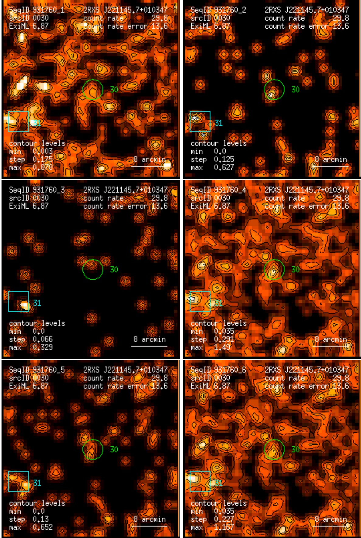
Figure 30: RASS 931760: detection 0030: band rate images, Gaussian filter: (1) PSPC channels 11 – 41, (2) 52 – 90, (3) 91 – 201, (4) 11 – 235, (5) 52 – 201, (6) 11 – 201. Broad band rates in counts/ks. Band rate contour levels in counts/ks/arcmin 2 .
