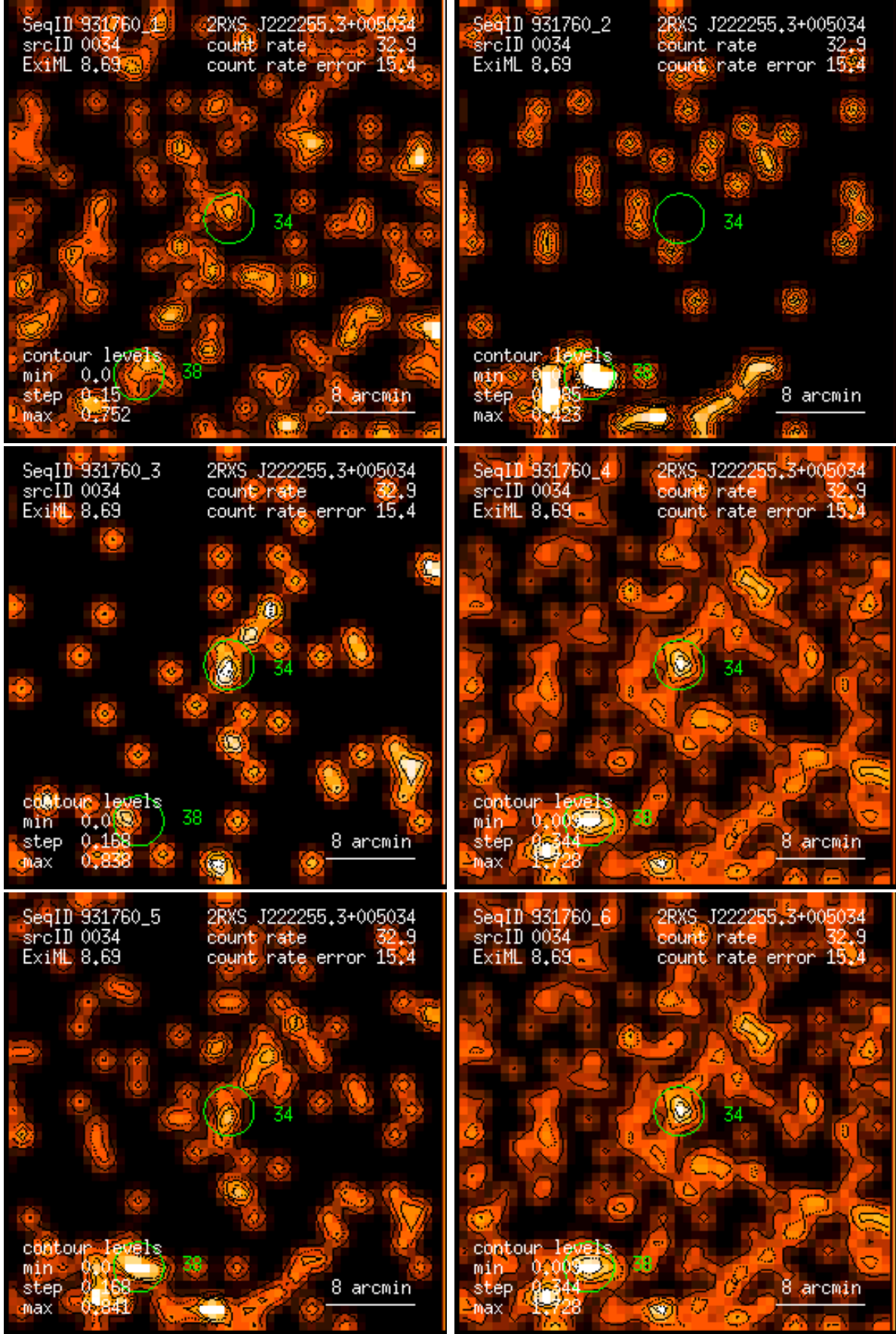
Figure 34: RASS 931760: detection 0034: band rate images, Gaussian filter: (1) PSPC channels 11 – 41, (2) 52 – 90, (3) 91 – 201, (4) 11 – 235, (5) 52 – 201, (6) 11 – 201. Broad band rates in counts/ks. Band rate contour levels in counts/ks/arcmin 2 .
