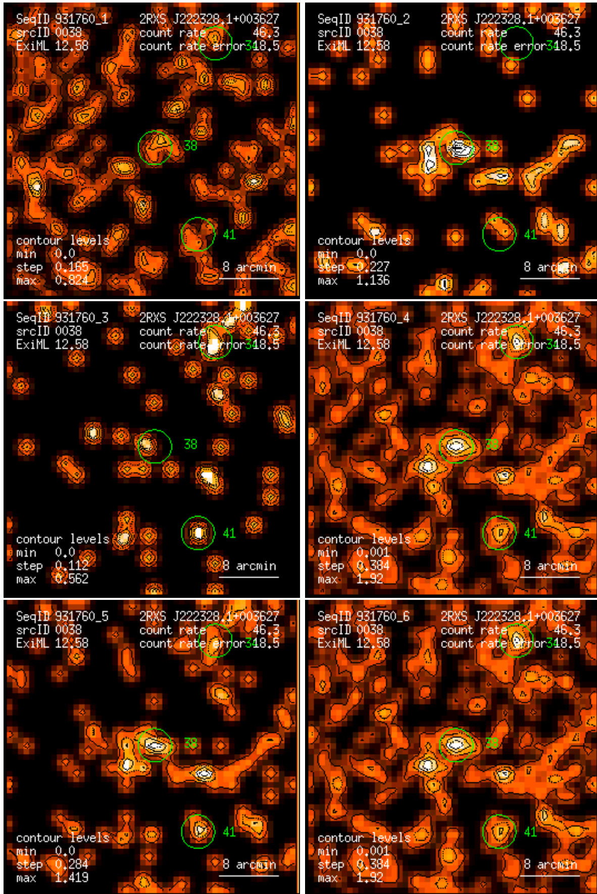
Figure 38: RASS 931760: detection 0038: band rate images, Gaussian filter: (1) PSPC channels 11 – 41, (2) 52 – 90, (3) 91 – 201, (4) 11 – 235, (5) 52 – 201, (6) 11 – 201. Broad band rates in counts/ks. Band rate contour levels in counts/ks/arcmin 2 .
