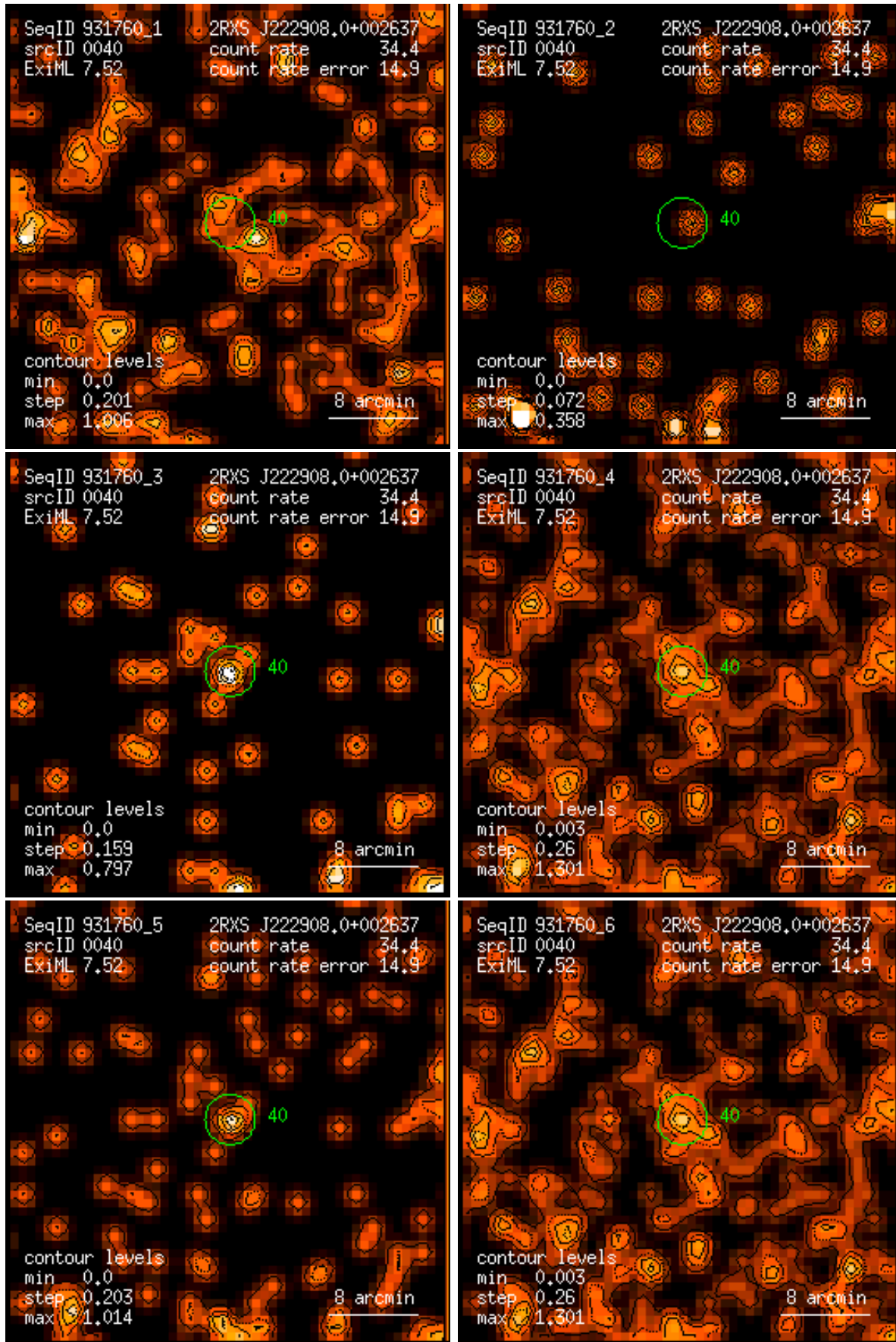
Figure 40: RASS 931760: detection 0040: band rate images, Gaussian filter: (1) PSPC channels 11 – 41, (2) 52 – 90, (3) 91 – 201, (4) 11 – 235, (5) 52 – 201, (6) 11 – 201. Broad band rates in counts/ks. Band rate contour levels in counts/ks/arcmin 2 .
