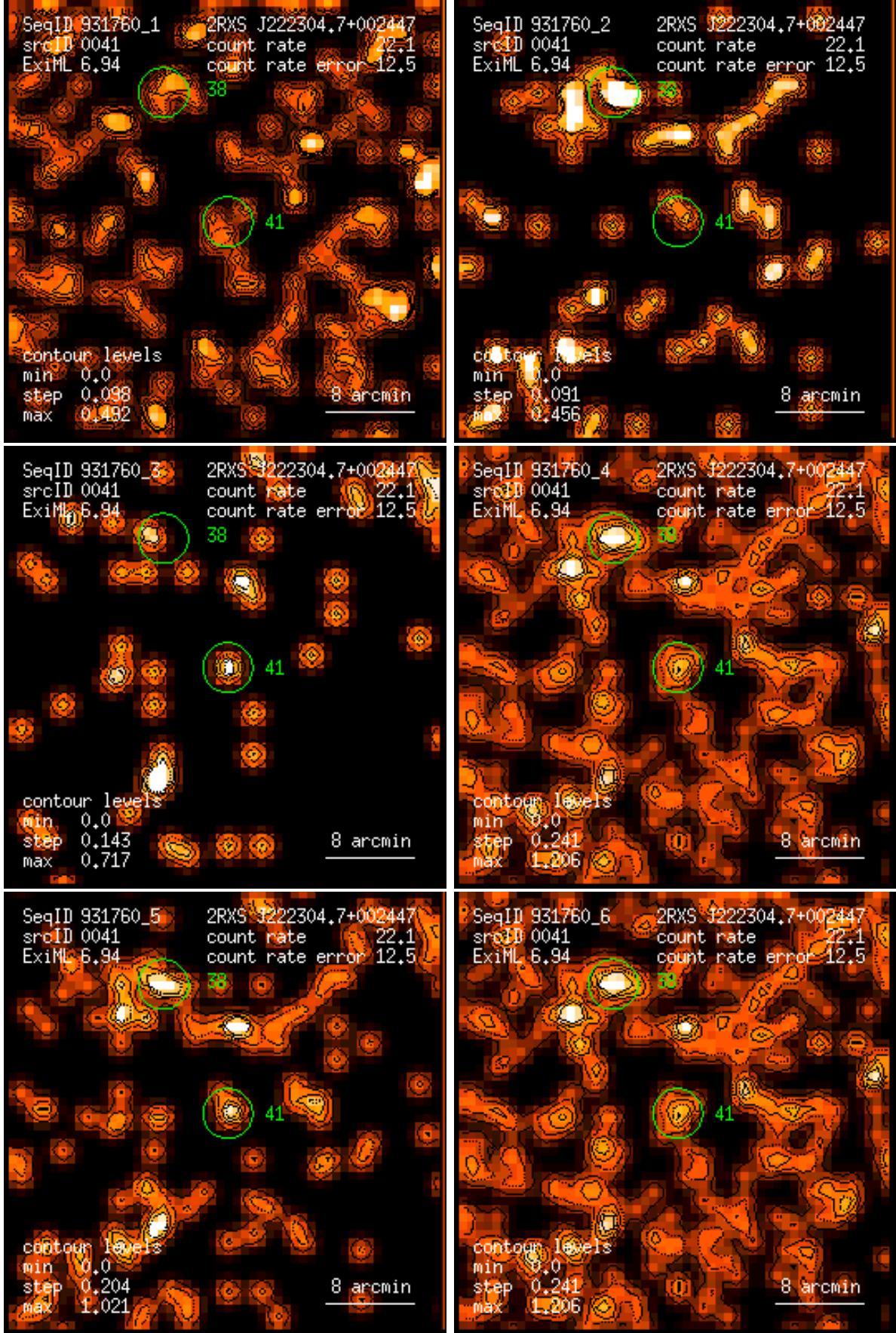
Figure 41: RASS 931760: detection 0041: band rate images, Gaussian filter: (1) PSPC channels 11 – 41, (2) 52 – 90, (3) 91 – 201, (4) 11 – 235, (5) 52 – 201, (6) 11 – 201. Broad band rates in counts/ks. Band rate contour levels in counts/ks/arcmin 2 .
