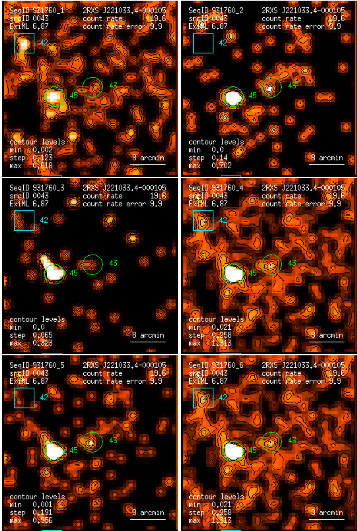
Figure 43: RASS 931760: detection 0043: band rate images, Gaussian filter: (1) PSPC channels 11 – 41, (2) 52 – 90, (3) 91 – 201, (4) 11 – 235, (5) 52 – 201, (6) 11 – 201. Broad band rates in counts/ks. Band rate contour levels in counts/ks/arcmin 2 .
