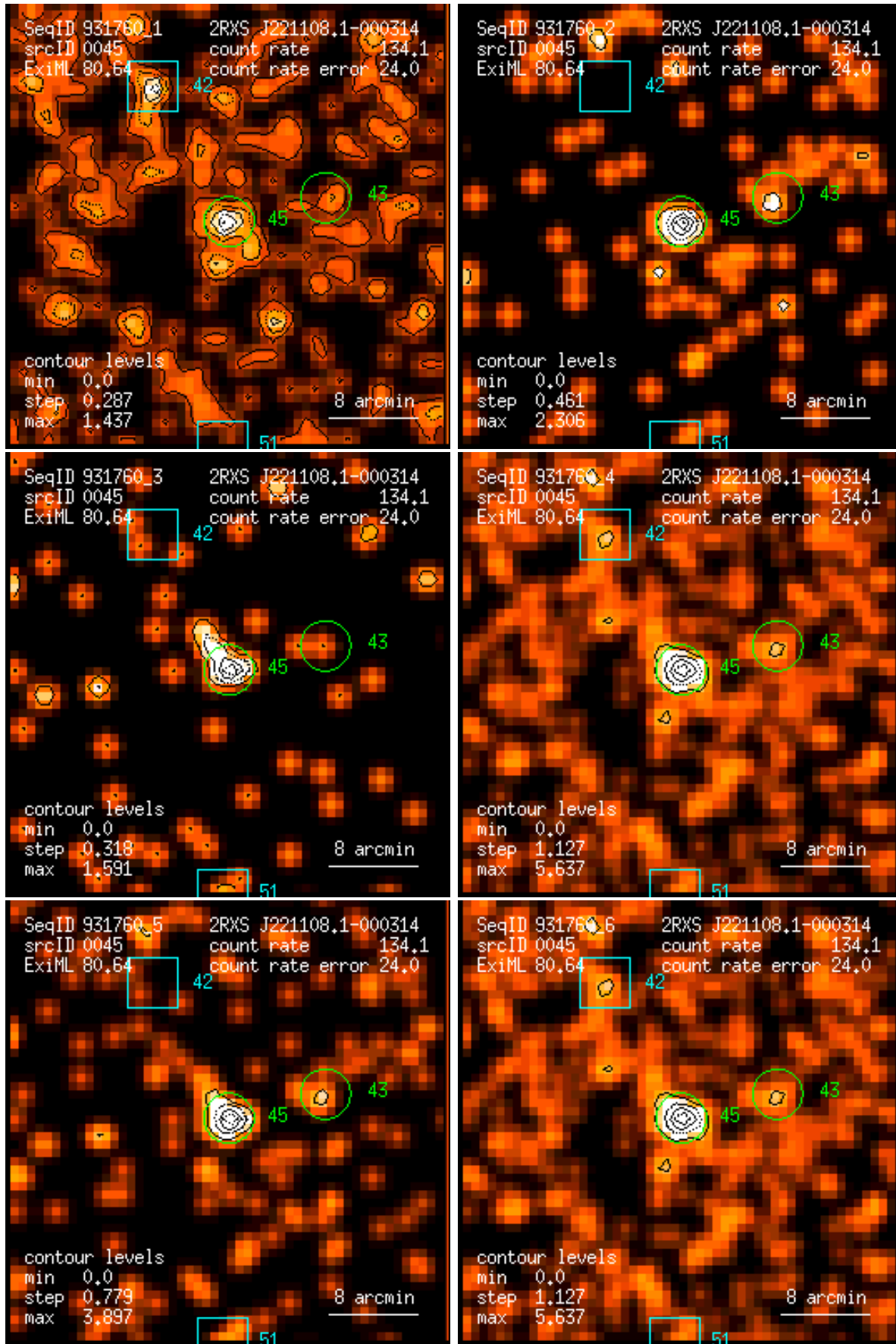
Figure 45: RASS 931760: detection 0045: band rate images, Gaussian filter: (1) PSPC channels 11 – 41, (2) 52 – 90, (3) 91 – 201, (4) 11 – 235, (5) 52 – 201, (6) 11 – 201. Broad band rates in counts/ks. Band rate contour levels in counts/ks/arcmin 2 .
