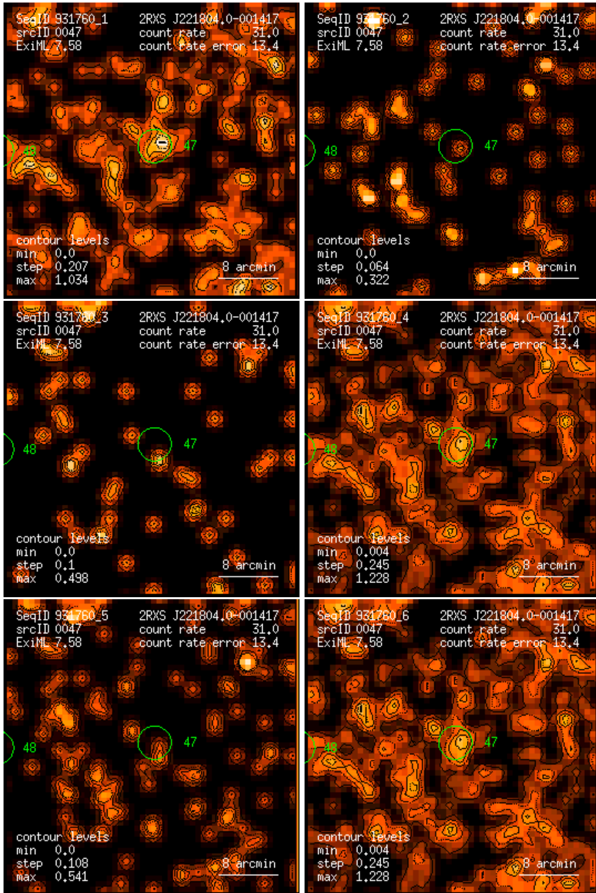
Figure 47: RASS 931760: detection 0047: band rate images, Gaussian filter: (1) PSPC channels 11 – 41, (2) 52 – 90, (3) 91 – 201, (4) 11 – 235, (5) 52 – 201, (6) 11 – 201. Broad band rates in counts/ks. Band rate contour levels in counts/ks/arcmin 2 .
