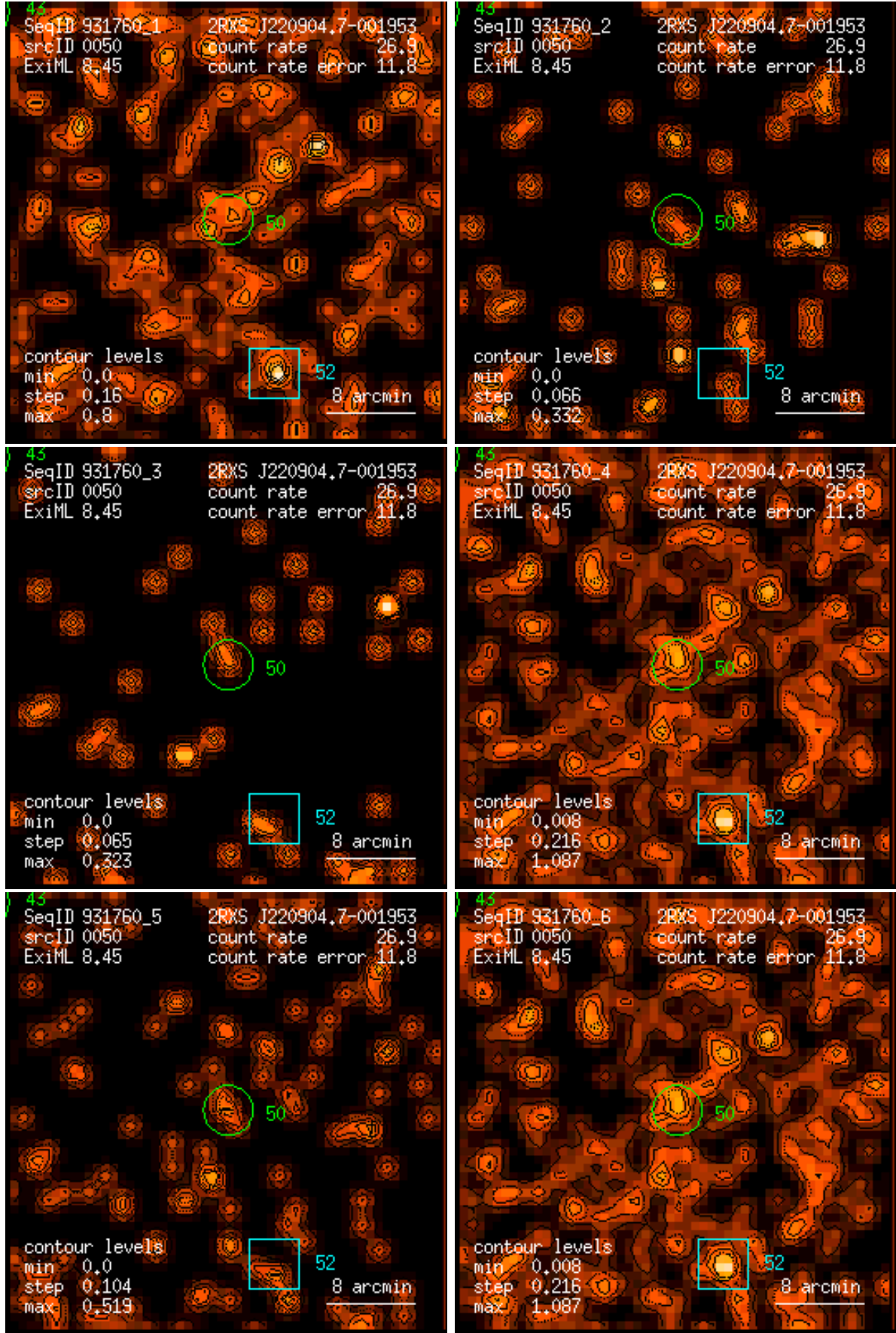
Figure 50: RASS 931760: detection 0050: band rate images, Gaussian filter: (1) PSPC channels 11 – 41, (2) 52 – 90, (3) 91 – 201, (4) 11 – 235, (5) 52 – 201, (6) 11 – 201. Broad band rates in counts/ks. Band rate contour levels in counts/ks/arcmin 2 .
