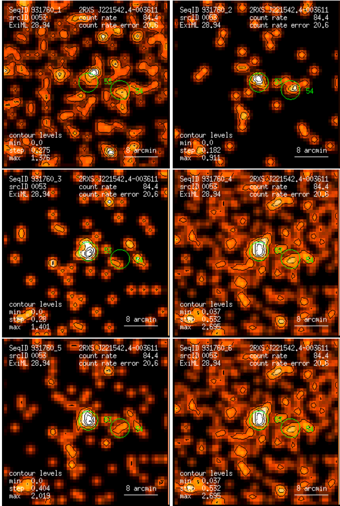
Figure 53: RASS 931760: detection 0053: band rate images, Gaussian filter: (1) PSPC channels 11 – 41, (2) 52 – 90, (3) 91 – 201, (4) 11 – 235, (5) 52 – 201, (6) 11 – 201. Broad band rates in counts/ks. Band rate contour levels in counts/ks/arcmin 2 .
