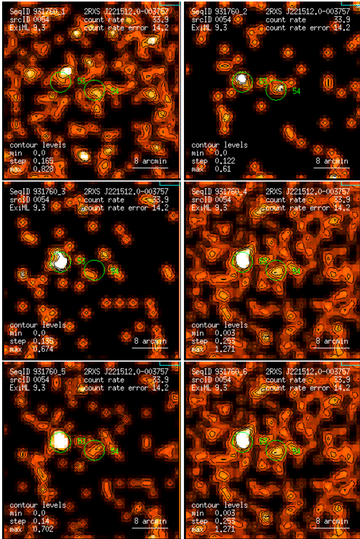
Figure 54: RASS 931760: detection 0054: band rate images, Gaussian filter: (1) PSPC channels 11 – 41, (2) 52 – 90, (3) 91 – 201, (4) 11 – 235, (5) 52 – 201, (6) 11 – 201. Broad band rates in counts/ks. Band rate contour levels in counts/ks/arcmin 2 .
