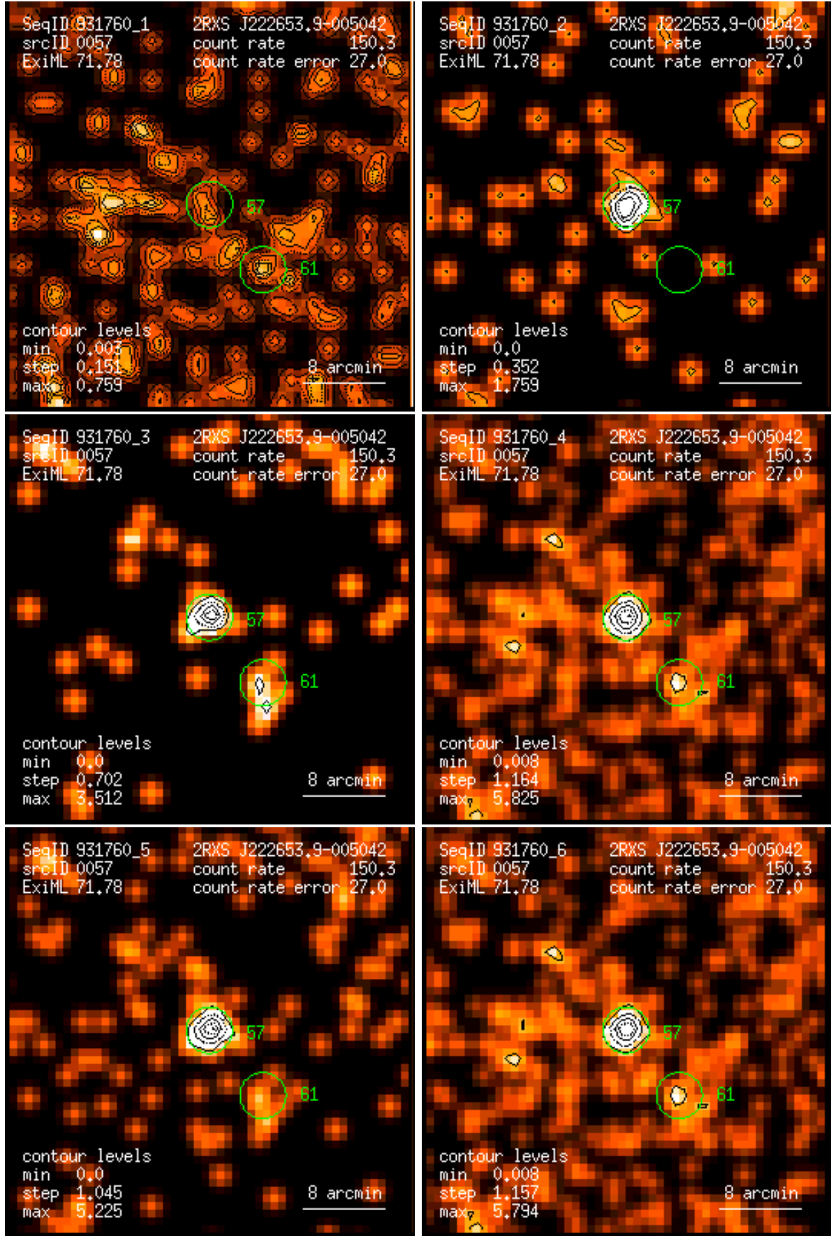
Figure 57: RASS 931760: detection 0057: band rate images, Gaussian filter: (1) PSPC channels 11 – 41, (2) 52 – 90, (3) 91 – 201, (4) 11 – 235, (5) 52 – 201, (6) 11 – 201. Broad band rates in counts/ks. Band rate contour levels in counts/ks/arcmin 2 .
