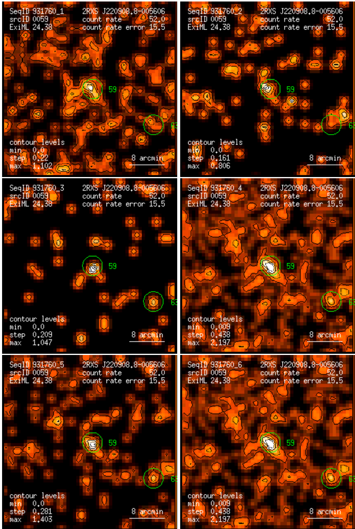
Figure 59: RASS 931760: detection 0059: band rate images, Gaussian filter: (1) PSPC channels 11 – 41, (2) 52 – 90, (3) 91 – 201, (4) 11 – 235, (5) 52 – 201, (6) 11 – 201. Broad band rates in counts/ks. Band rate contour levels in counts/ks/arcmin 2 .
