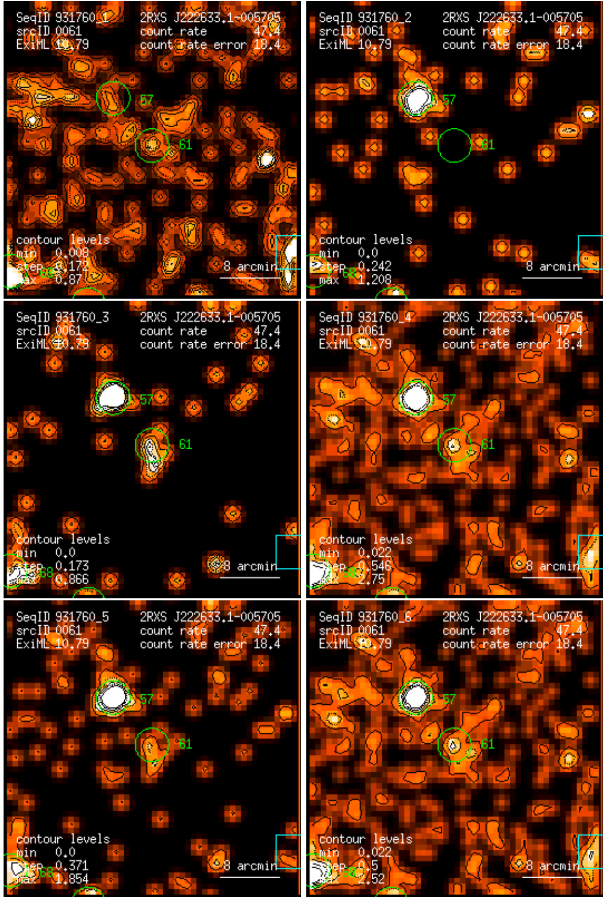
Figure 61: RASS 931760: detection 0061: band rate images, Gaussian filter: (1) PSPC channels 11 – 41, (2) 52 – 90, (3) 91 – 201, (4) 11 – 235, (5) 52 – 201, (6) 11 – 201. Broad band rates in counts/ks. Band rate contour levels in counts/ks/arcmin 2 .
