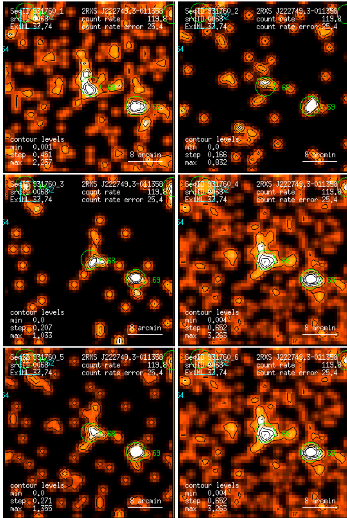
Figure 68: RASS 931760: detection 0068: band rate images, Gaussian filter: (1) PSPC channels 11 – 41, (2) 52 – 90, (3) 91 – 201, (4) 11 – 235, (5) 52 – 201, (6) 11 – 201. Broad band rates in counts/ks. Band rate contour levels in counts/ks/arcmin 2 .
