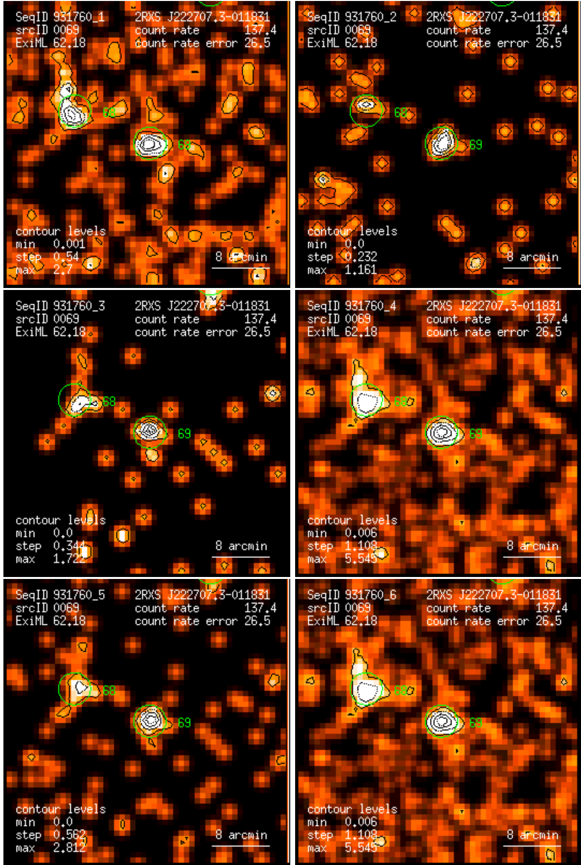
Figure 69: RASS 931760: detection 0069: band rate images, Gaussian filter: (1) PSPC channels 11 – 41, (2) 52 – 90, (3) 91 – 201, (4) 11 – 235, (5) 52 – 201, (6) 11 – 201. Broad band rates in counts/ks. Band rate contour levels in counts/ks/arcmin 2 .
