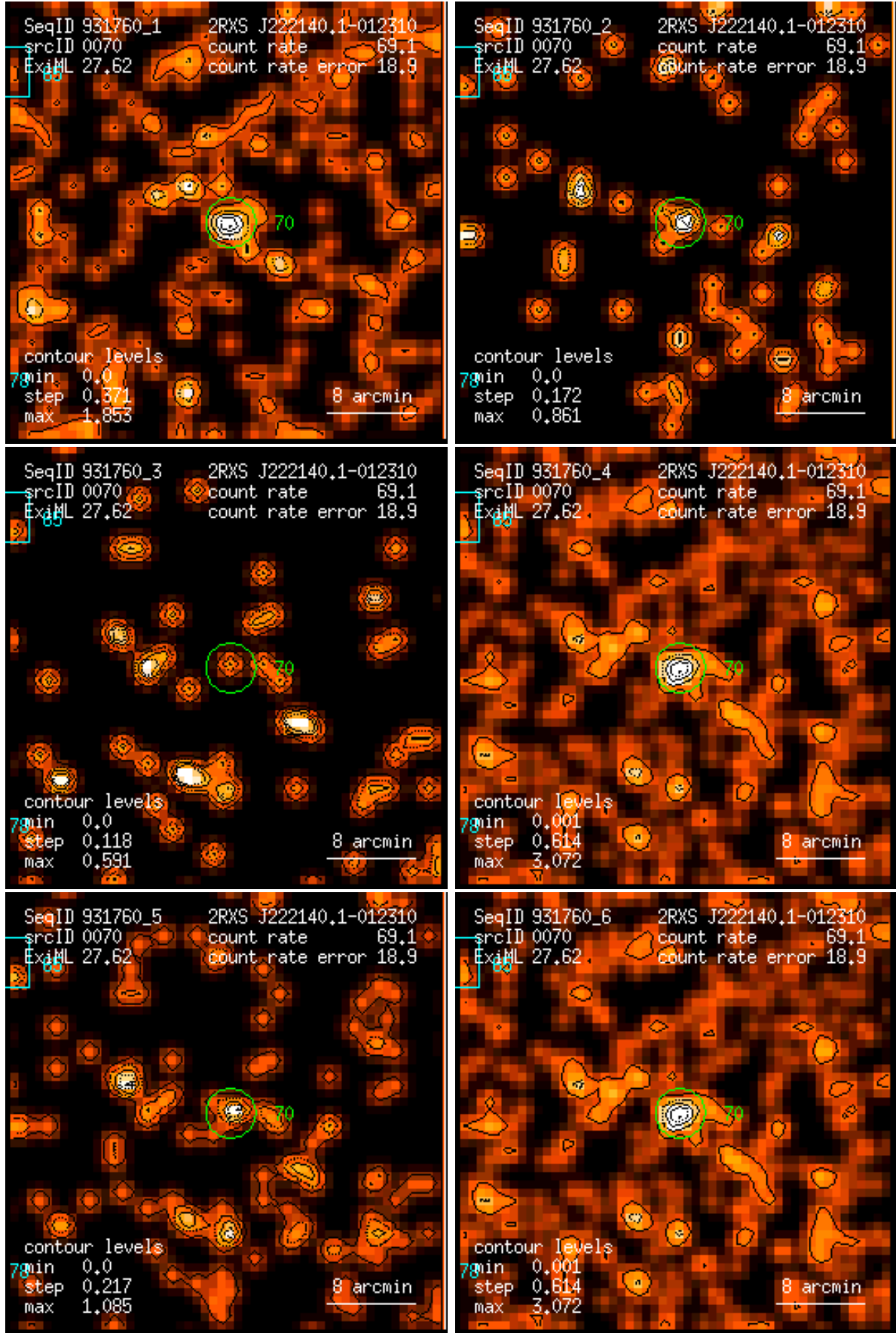
Figure 70: RASS 931760: detection 0070: band rate images, Gaussian filter: (1) PSPC channels 11 – 41, (2) 52 – 90, (3) 91 – 201, (4) 11 – 235, (5) 52 – 201, (6) 11 – 201. Broad band rates in counts/ks. Band rate contour levels in counts/ks/arcmin 2 .
