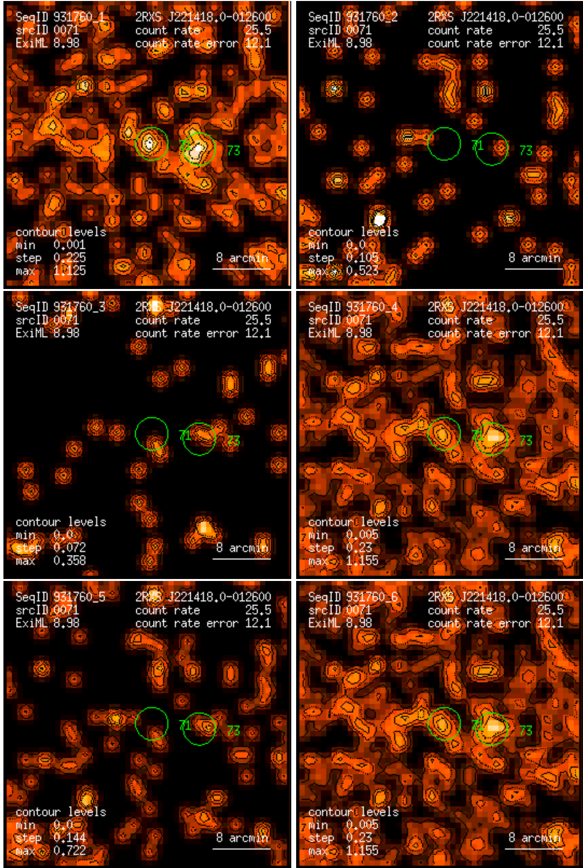
Figure 71: RASS 931760: detection 0071: band rate images, Gaussian filter: (1) PSPC channels 11 – 41, (2) 52 – 90, (3) 91 – 201, (4) 11 – 235, (5) 52 – 201, (6) 11 – 201. Broad band rates in counts/ks. Band rate contour levels in counts/ks/arcmin 2 .
