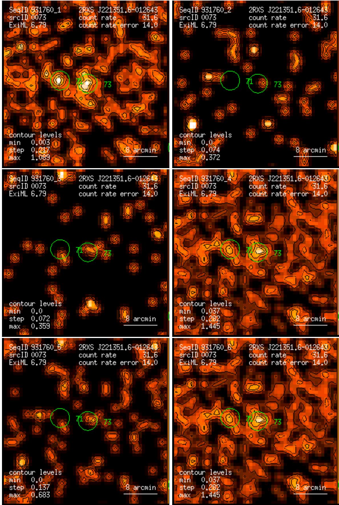
Figure 73: RASS 931760: detection 0073: band rate images, Gaussian filter: (1) PSPC channels 11 – 41, (2) 52 – 90, (3) 91 – 201, (4) 11 – 235, (5) 52 – 201, (6) 11 – 201. Broad band rates in counts/ks. Band rate contour levels in counts/ks/arcmin 2 .
