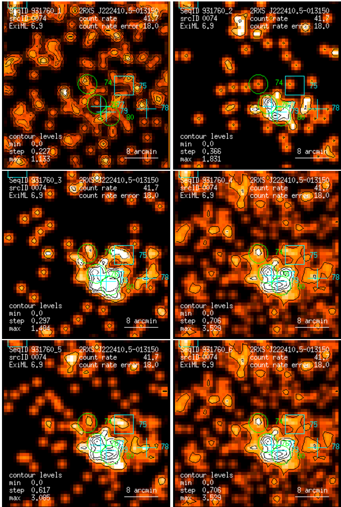
Figure 74: RASS 931760: detection 0074: band rate images, Gaussian filter: (1) PSPC channels 11 – 41, (2) 52 – 90, (3) 91 – 201, (4) 11 – 235, (5) 52 – 201, (6) 11 – 201. Broad band rates in counts/ks. Band rate contour levels in counts/ks/arcmin 2 .
