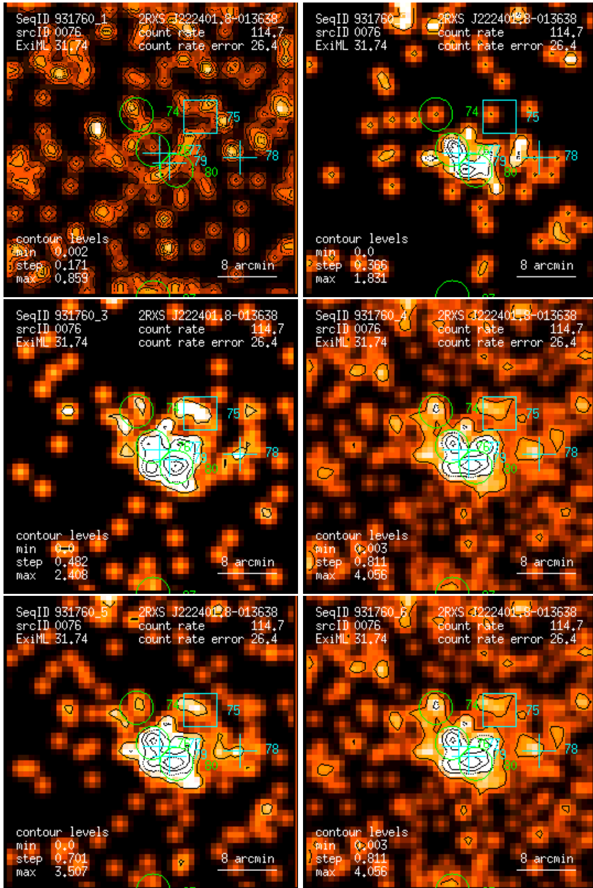
Figure 76: RASS 931760: detection 0076: band rate images, Gaussian filter: (1) PSPC channels 11 – 41, (2) 52 – 90, (3) 91 – 201, (4) 11 – 235, (5) 52 – 201, (6) 11 – 201. Broad band rates in counts/ks. Band rate contour levels in counts/ks/arcmin 2 .
