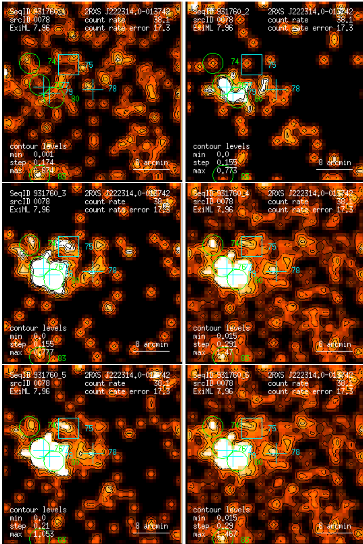
Figure 78: RASS 931760: detection 0078: band rate images, Gaussian filter: (1) PSPC channels 11 – 41, (2) 52 – 90, (3) 91 – 201, (4) 11 – 235, (5) 52 – 201, (6) 11 – 201. Broad band rates in counts/ks. Band rate contour levels in counts/ks/arcmin 2 .
