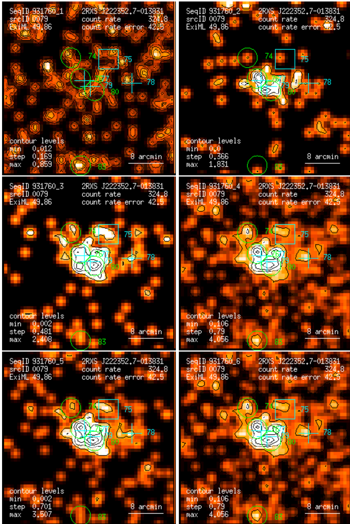
Figure 79: RASS 931760: detection 0079: band rate images, Gaussian filter: (1) PSPC channels 11 – 41, (2) 52 – 90, (3) 91 – 201, (4) 11 – 235, (5) 52 – 201, (6) 11 – 201. Broad band rates in counts/ks. Band rate contour levels in counts/ks/arcmin 2 .
