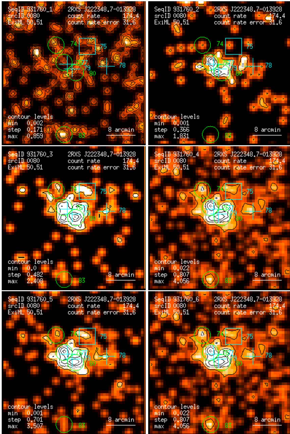
Figure 80: RASS 931760: detection 0080: band rate images, Gaussian filter: (1) PSPC channels 11 – 41, (2) 52 – 90, (3) 91 – 201, (4) 11 – 235, (5) 52 – 201, (6) 11 – 201. Broad band rates in counts/ks. Band rate contour levels in counts/ks/arcmin 2 .
