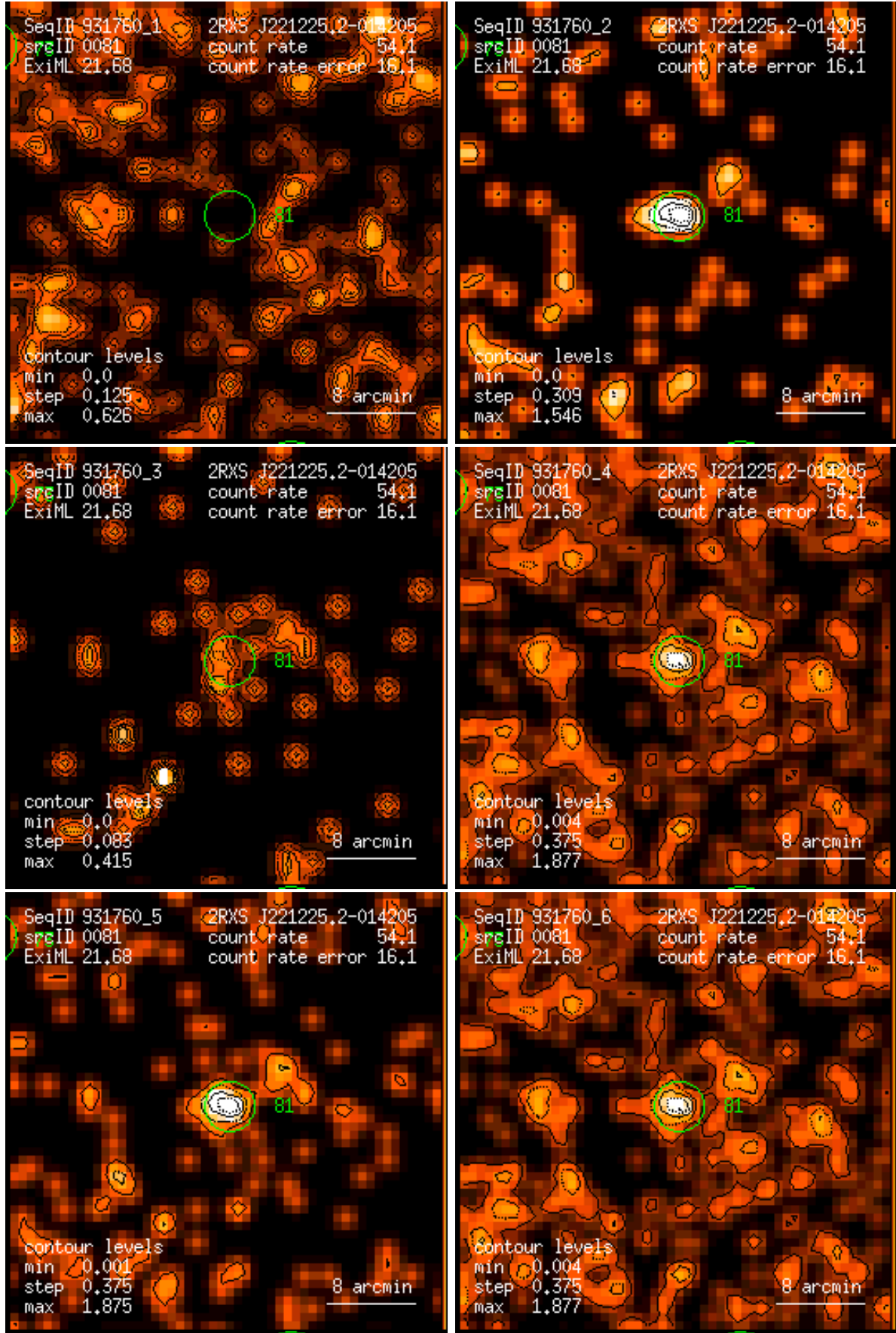
Figure 81: RASS 931760: detection 0081: band rate images, Gaussian filter: (1) PSPC channels 11 – 41, (2) 52 – 90, (3) 91 – 201, (4) 11 – 235, (5) 52 – 201, (6) 11 – 201. Broad band rates in counts/ks. Band rate contour levels in counts/ks/arcmin 2 .
