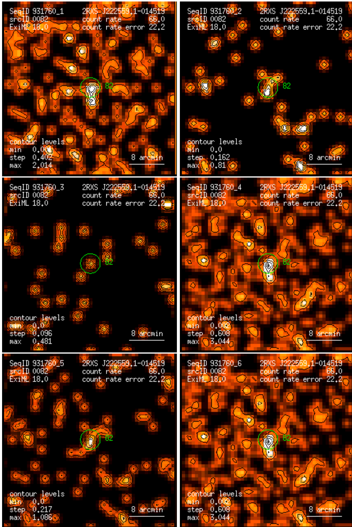
Figure 82: RASS 931760: detection 0082: band rate images, Gaussian filter: (1) PSPC channels 11 – 41, (2) 52 – 90, (3) 91 – 201, (4) 11 – 235, (5) 52 – 201, (6) 11 – 201. Broad band rates in counts/ks. Band rate contour levels in counts/ks/arcmin 2 .
