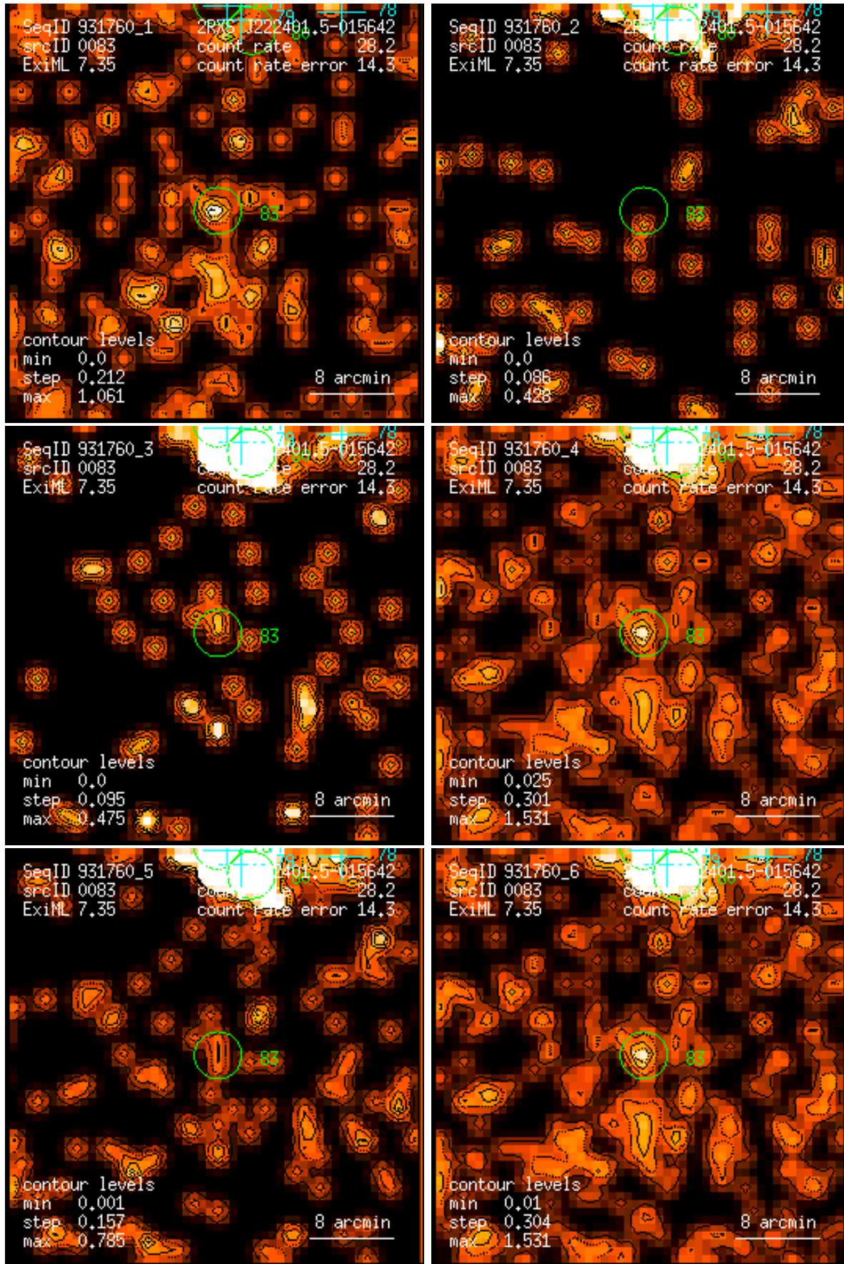
Figure 83: RASS 931760: detection 0083: band rate images, Gaussian filter: (1) PSPC channels 11 – 41, (2) 52 – 90, (3) 91 – 201, (4) 11 – 235, (5) 52 – 201, (6) 11 – 201. Broad band rates in counts/ks. Band rate contour levels in counts/ks/arcmin 2 .
