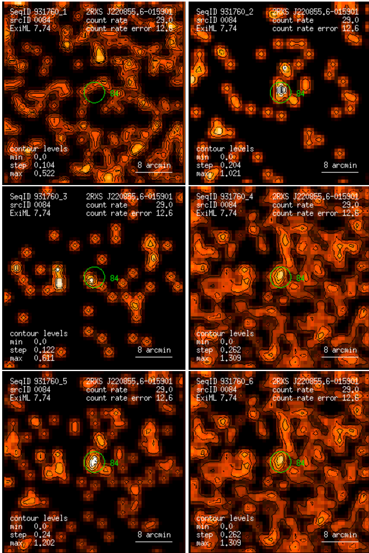
Figure 84: RASS 931760: detection 0084: band rate images, Gaussian filter: (1) PSPC channels 11 – 41, (2) 52 – 90, (3) 91 – 201, (4) 11 – 235, (5) 52 – 201, (6) 11 – 201. Broad band rates in counts/ks. Band rate contour levels in counts/ks/arcmin 2 .
