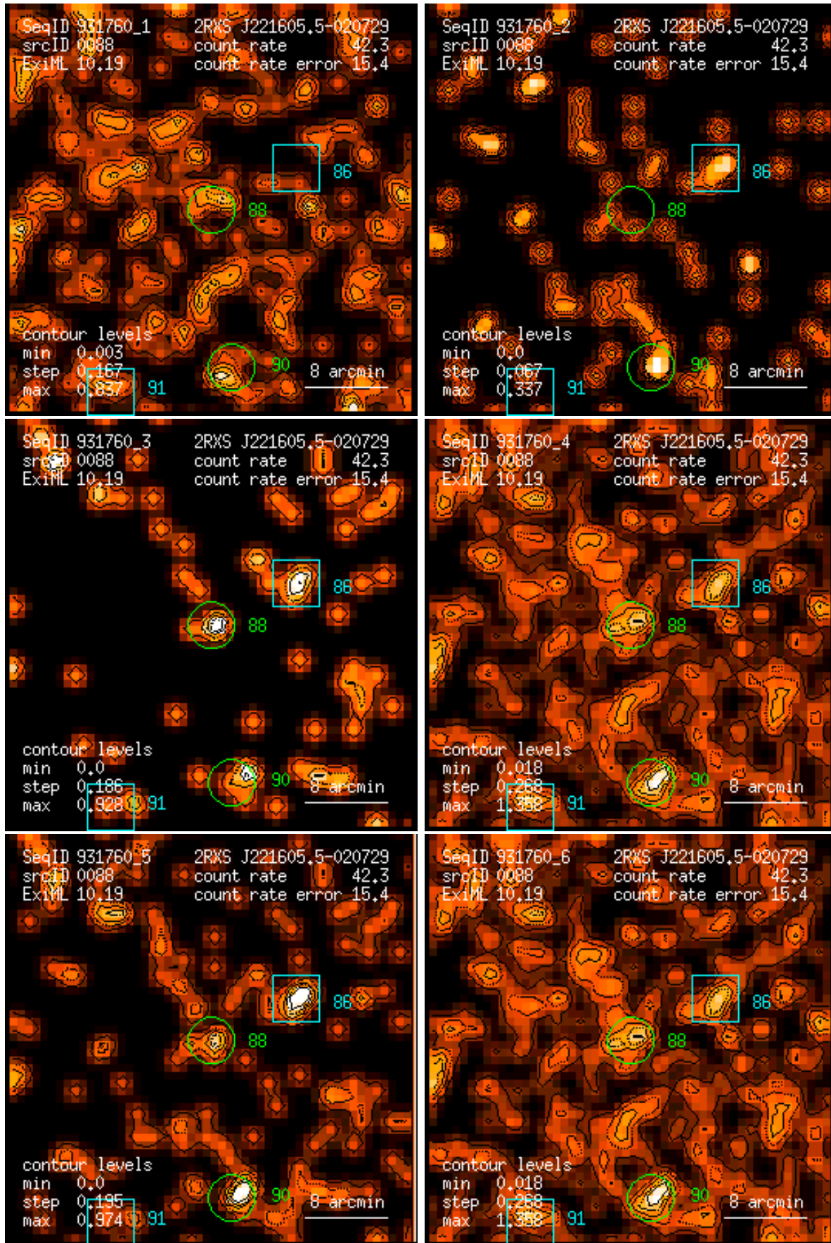
Figure 88: RASS 931760: detection 0088: band rate images, Gaussian filter: (1) PSPC channels 11 – 41, (2) 52 – 90, (3) 91 – 201, (4) 11 – 235, (5) 52 – 201, (6) 11 – 201. Broad band rates in counts/ks. Band rate contour levels in counts/ks/arcmin 2 .
