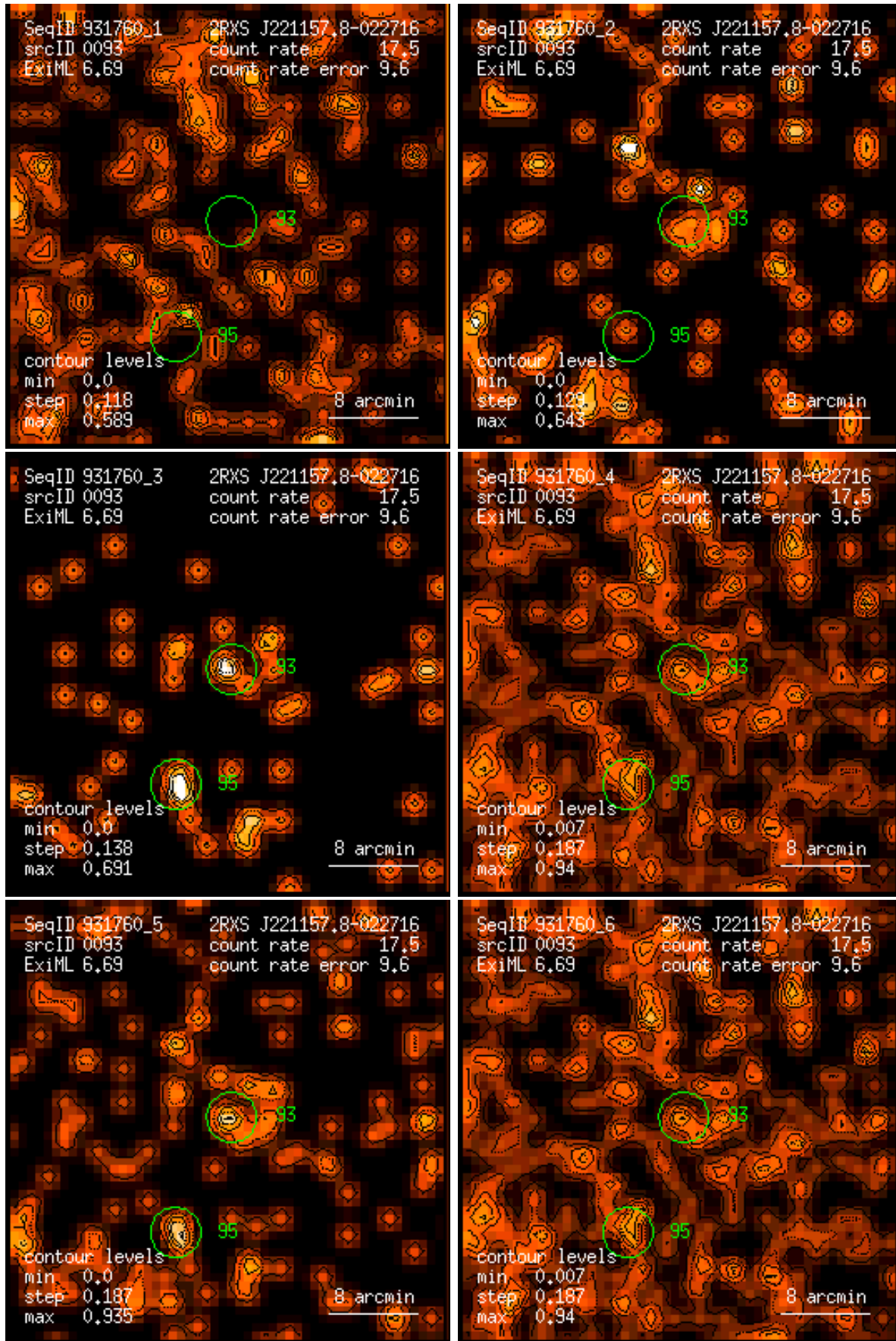
Figure 93: RASS 931760: detection 0093: band rate images, Gaussian filter: (1) PSPC channels 11 – 41, (2) 52 – 90, (3) 91 – 201, (4) 11 – 235, (5) 52 – 201, (6) 11 – 201. Broad band rates in counts/ks. Band rate contour levels in counts/ks/arcmin 2 .
