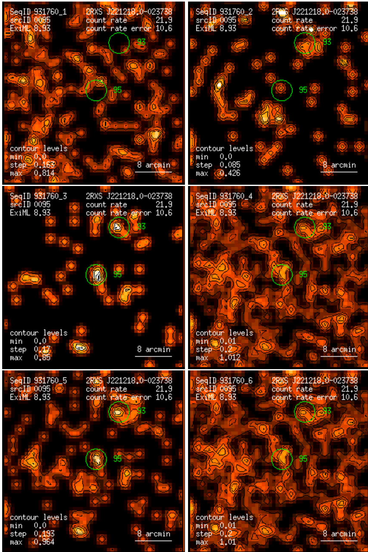
Figure 95: RASS 931760: detection 0095: band rate images, Gaussian filter: (1) PSPC channels 11 – 41, (2) 52 – 90, (3) 91 – 201, (4) 11 – 235, (5) 52 – 201, (6) 11 – 201. Broad band rates in counts/ks. Band rate contour levels in counts/ks/arcmin 2 .
