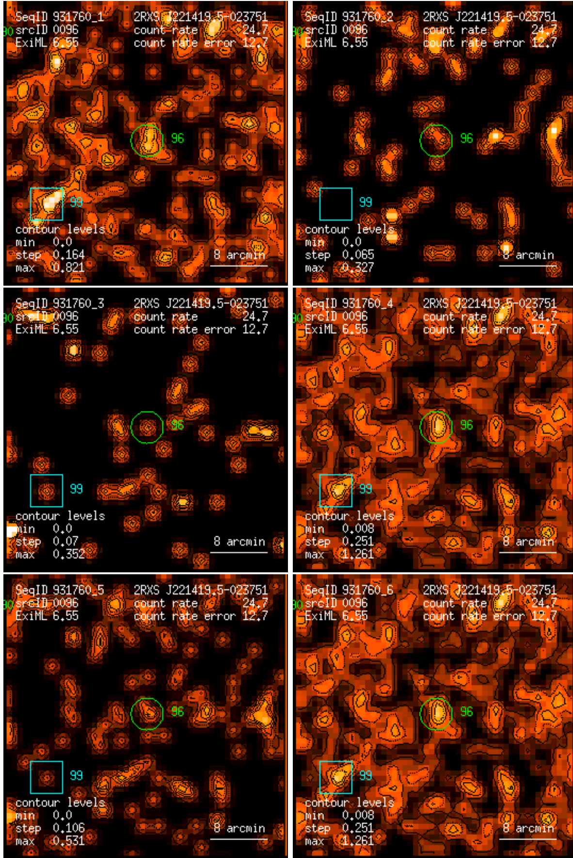
Figure 96: RASS 931760: detection 0096: band rate images, Gaussian filter: (1) PSPC channels 11 – 41, (2) 52 – 90, (3) 91 – 201, (4) 11 – 235, (5) 52 – 201, (6) 11 – 201. Broad band rates in counts/ks. Band rate contour levels in counts/ks/arcmin 2 .
