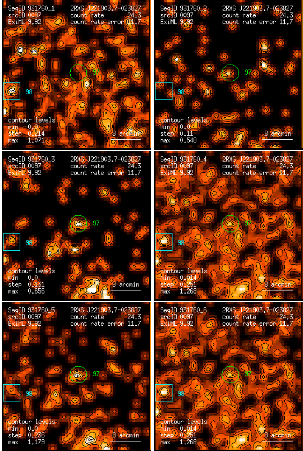
Figure 97: RASS 931760: detection 0097: band rate images, Gaussian filter: (1) PSPC channels 11 – 41, (2) 52 – 90, (3) 91 – 201, (4) 11 – 235, (5) 52 – 201, (6) 11 – 201. Broad band rates in counts/ks. Band rate contour levels in counts/ks/arcmin 2 .
