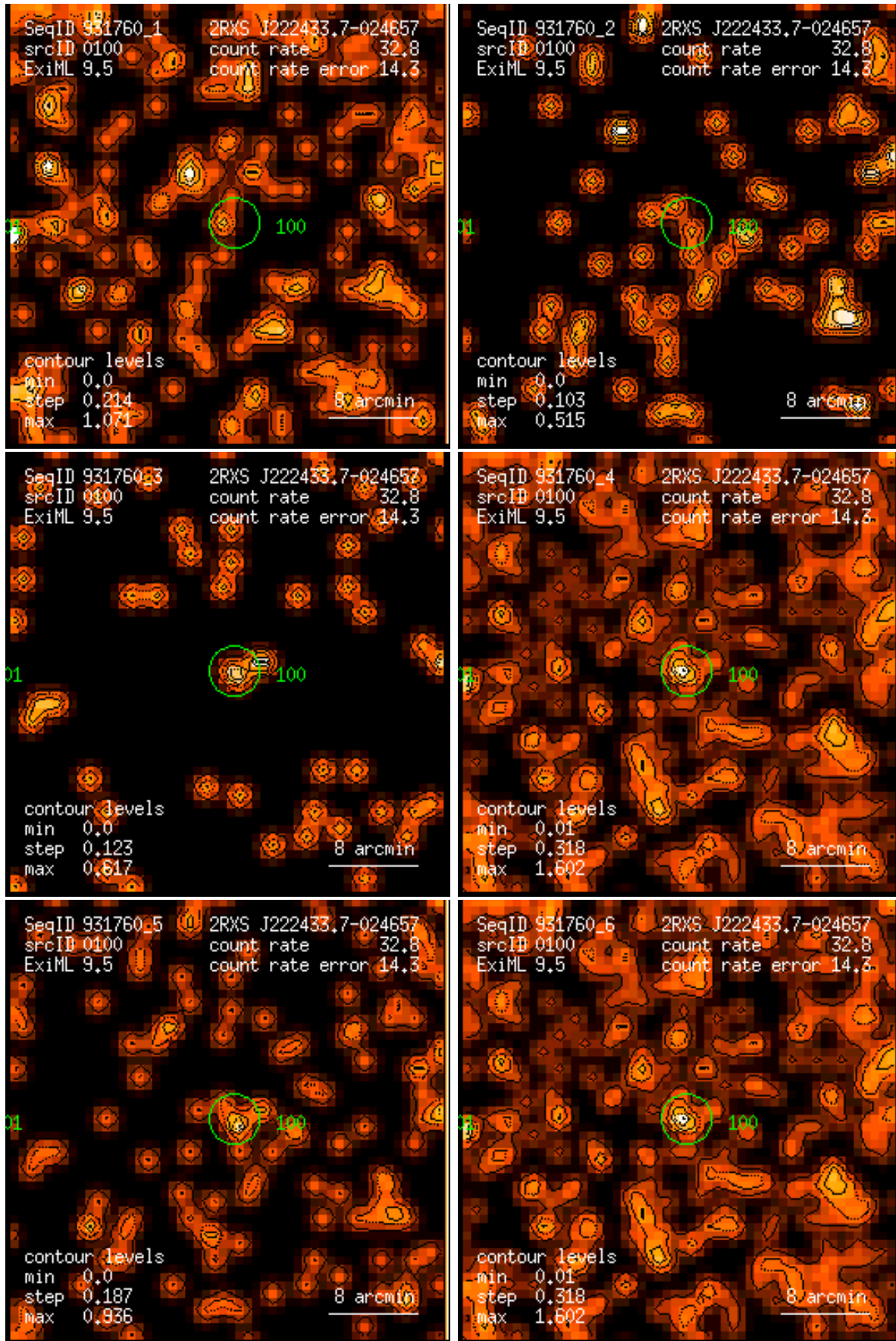
Figure 100: RASS 931760: detection 0100: band rate images, Gaussian filter: (1) PSPC channels 11 – 41, (2) 52 – 90, (3) 91 – 201, (4) 11 – 235, (5) 52 – 201, (6) 11 – 201. Broad band rates in counts/ks. Band rate contour levels in counts/ks/arcmin 2 .
