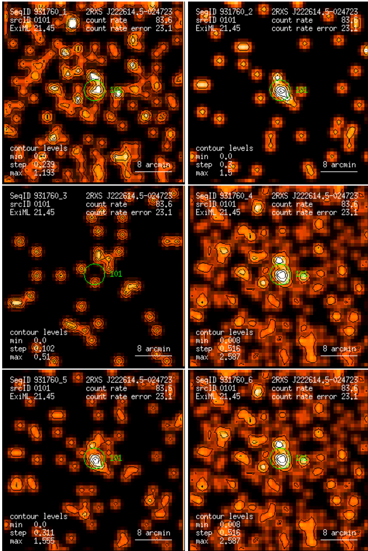
Figure 101: RASS 931760: detection 0101: band rate images, Gaussian filter: (1) PSPC channels 11 – 41, (2) 52 – 90, (3) 91 – 201, (4) 11 – 235, (5) 52 – 201, (6) 11 – 201. Broad band rates in counts/ks. Band rate contour levels in counts/ks/arcmin 2 .
