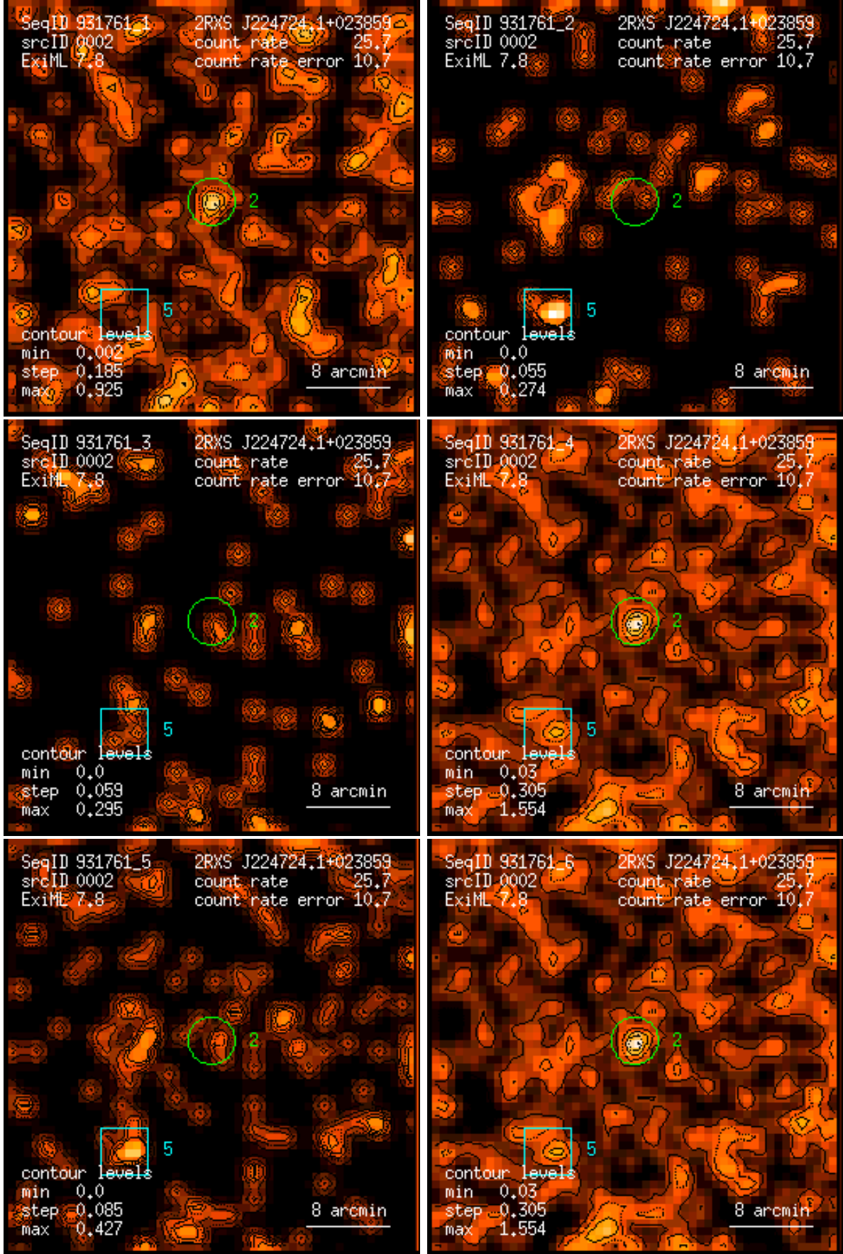
Figure 2: RASS 931761: detection 0002: band rate images, Gaussian filter: (1) PSPC channels 11 – 41, (2) 52 – 90, (3) 91 – 201, (4) 11 – 235, (5) 52 – 201, (6) 11 – 201. Broad band rates in counts/ks. Band rate contour levels in counts/ks/arcmin 2 .
