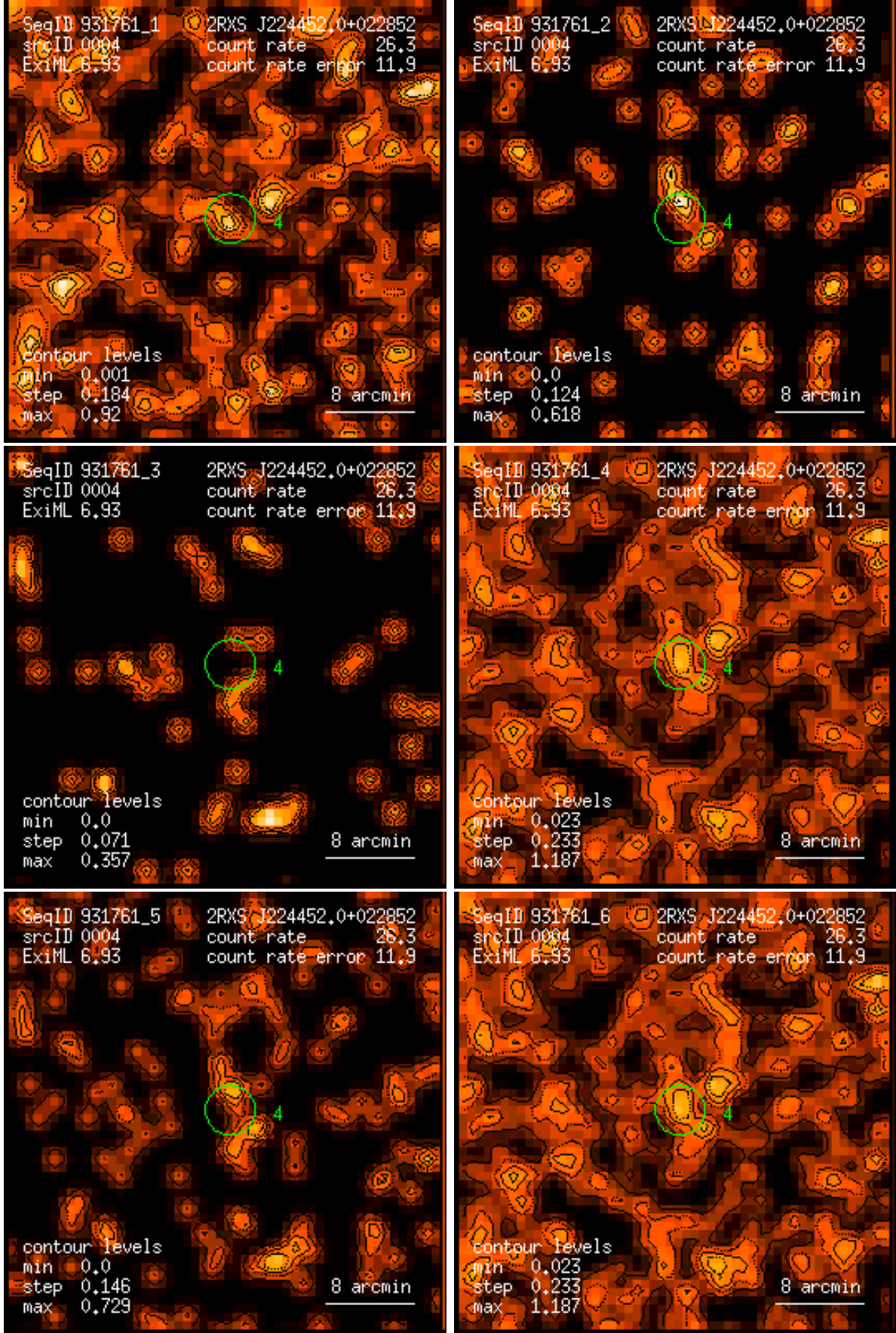
Figure 4: RASS 931761: detection 0004: band rate images, Gaussian filter: (1) PSPC channels 11 – 41, (2) 52 – 90, (3) 91 – 201, (4) 11 – 235, (5) 52 – 201, (6) 11 – 201. Broad band rates in counts/ks. Band rate contour levels in counts/ks/arcmin 2 .
