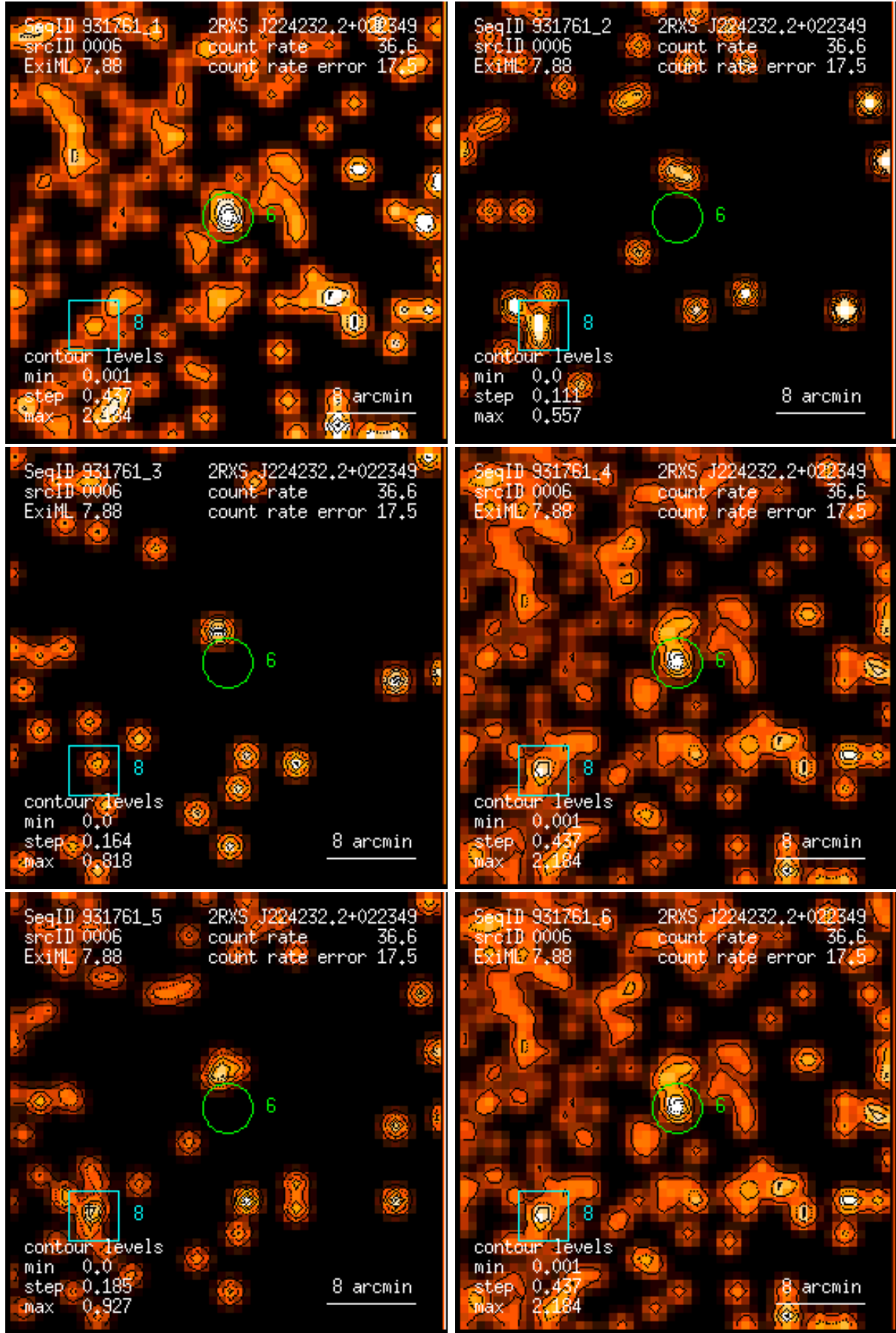
Figure 6: RASS 931761: detection 0006: band rate images, Gaussian filter: (1) PSPC channels 11 – 41, (2) 52 – 90, (3) 91 – 201, (4) 11 – 235, (5) 52 – 201, (6) 11 – 201. Broad band rates in counts/ks. Band rate contour levels in counts/ks/arcmin 2 .
