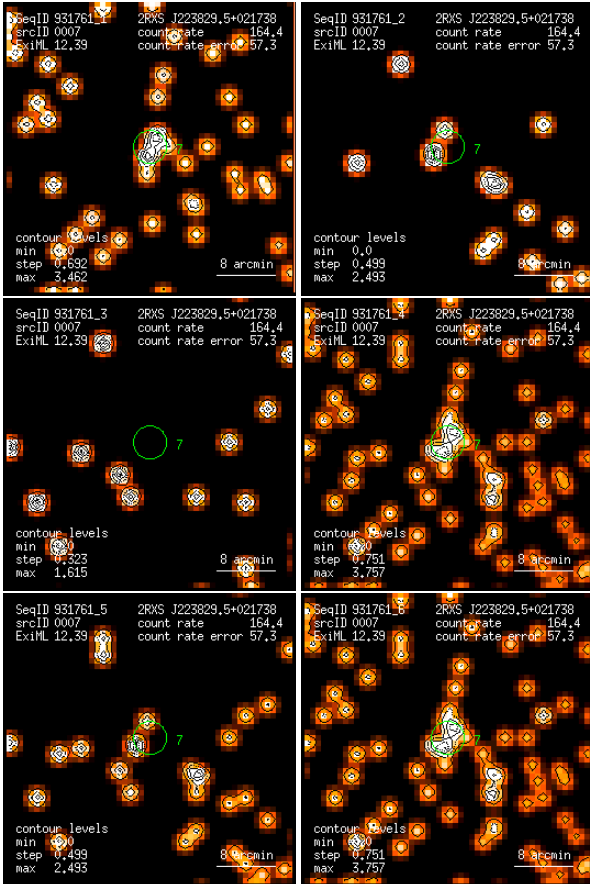
Figure 7: RASS 931761: detection 0007: band rate images, Gaussian filter: (1) PSPC channels 11 – 41, (2) 52 – 90, (3) 91 – 201, (4) 11 – 235, (5) 52 – 201, (6) 11 – 201. Broad band rates in counts/ks. Band rate contour levels in counts/ks/arcmin 2 .
