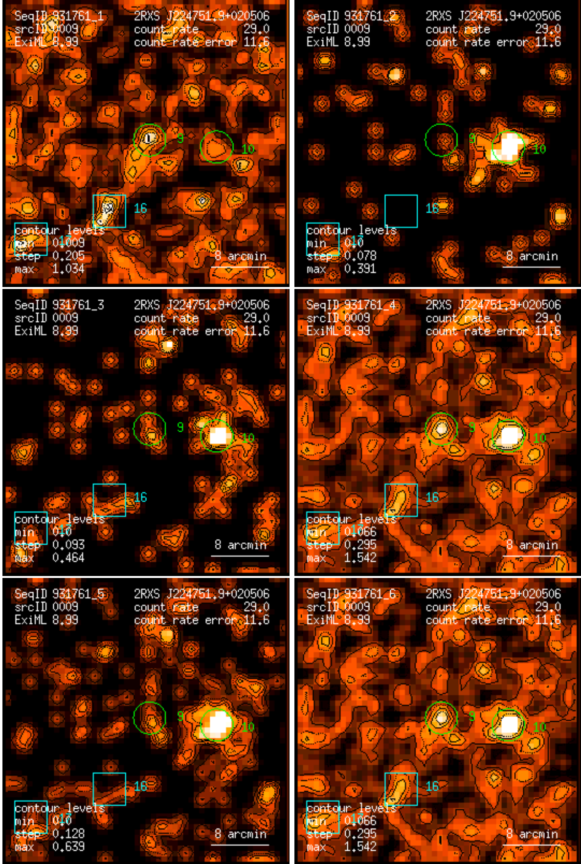
Figure 9: RASS 931761: detection 0009: band rate images, Gaussian filter: (1) PSPC channels 11 – 41, (2) 52 – 90, (3) 91 – 201, (4) 11 – 235, (5) 52 – 201, (6) 11 – 201. Broad band rates in counts/ks. Band rate contour levels in counts/ks/arcmin 2 .
