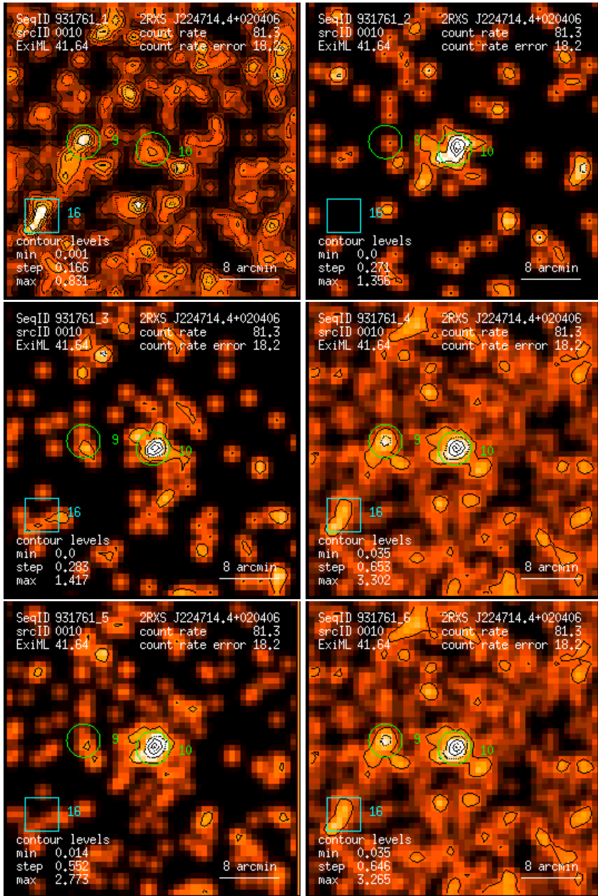
Figure 10: RASS 931761: detection 0010: band rate images, Gaussian filter: (1) PSPC channels 11 – 41, (2) 52 – 90, (3) 91 – 201, (4) 11 – 235, (5) 52 – 201, (6) 11 – 201. Broad band rates in counts/ks. Band rate contour levels in counts/ks/arcmin 2 .
